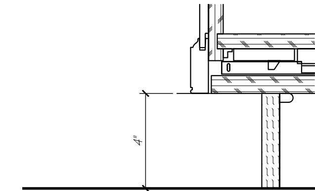
TOE DETAIL
