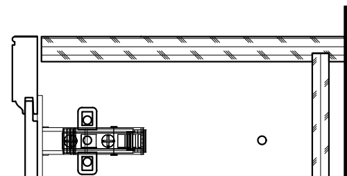
CROWN DETAIL
