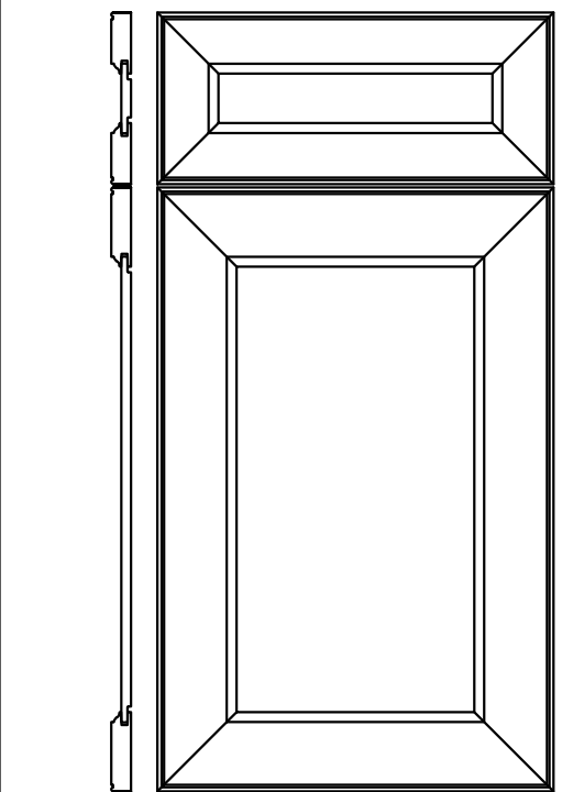
DOOR DETAIL SCALE: 1 1/2" = 1'-0"
