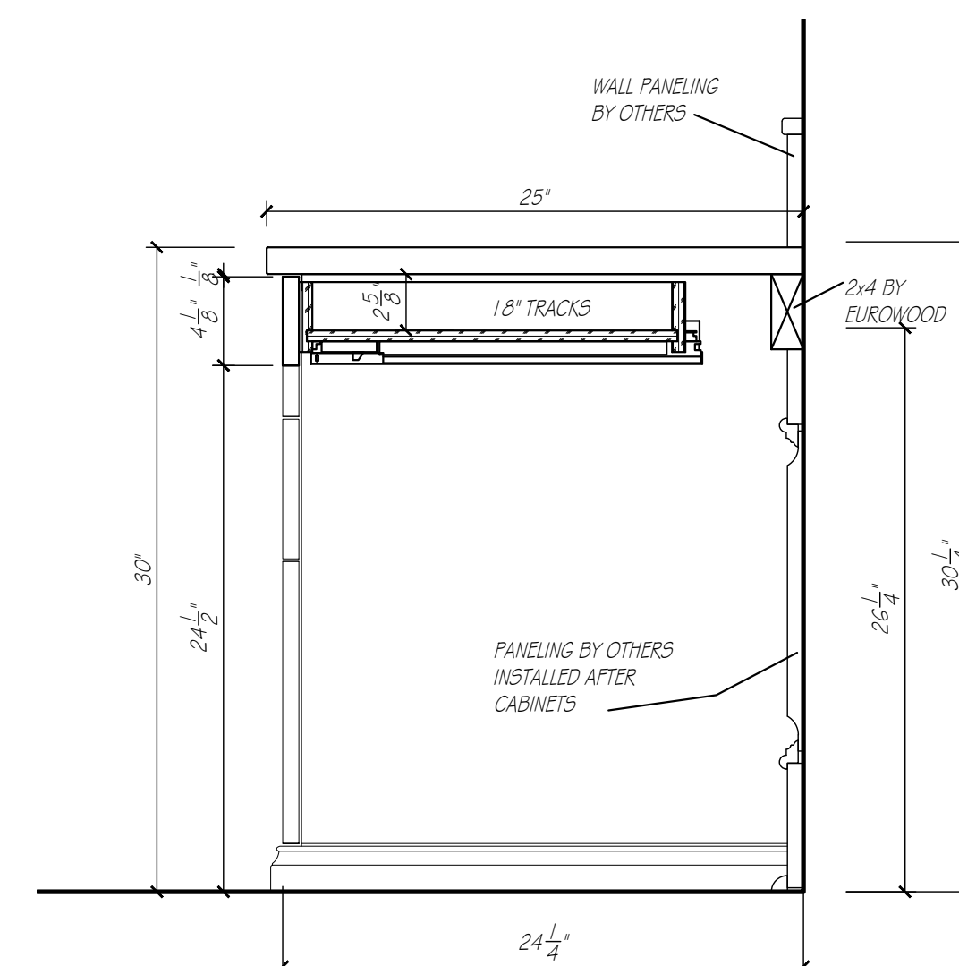
7 CABINET DETAIL A9 SCALE: 1 1/2" = 1'-0"
