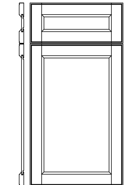
DOOR DETAIL ✓ EW-CWS SCALE: 1 1/2" = 1'-0"
