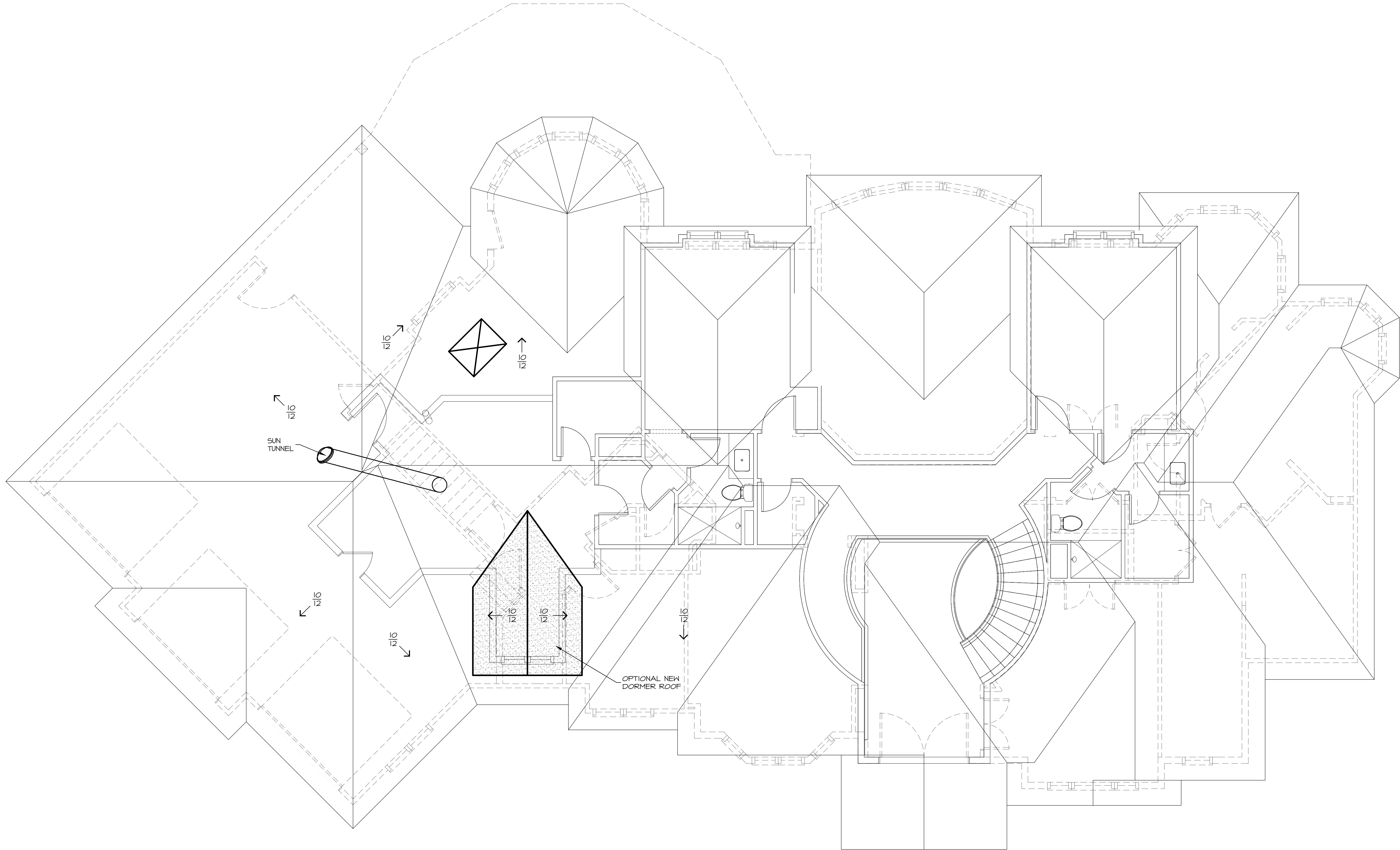
ROOF PLAN 1/4" = 1'-0"
