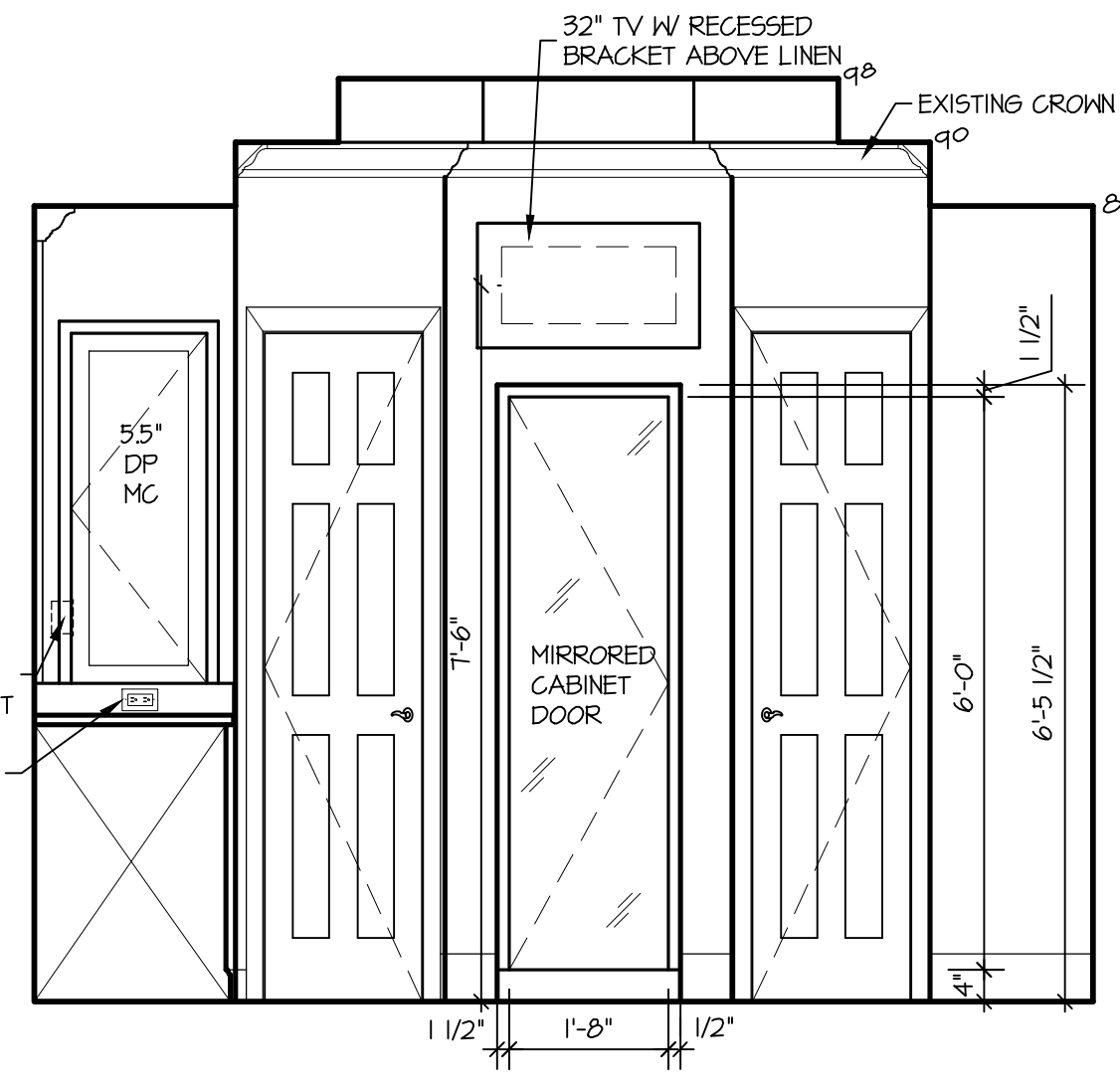
04 PRIMARY BATH 1/2\"/>
