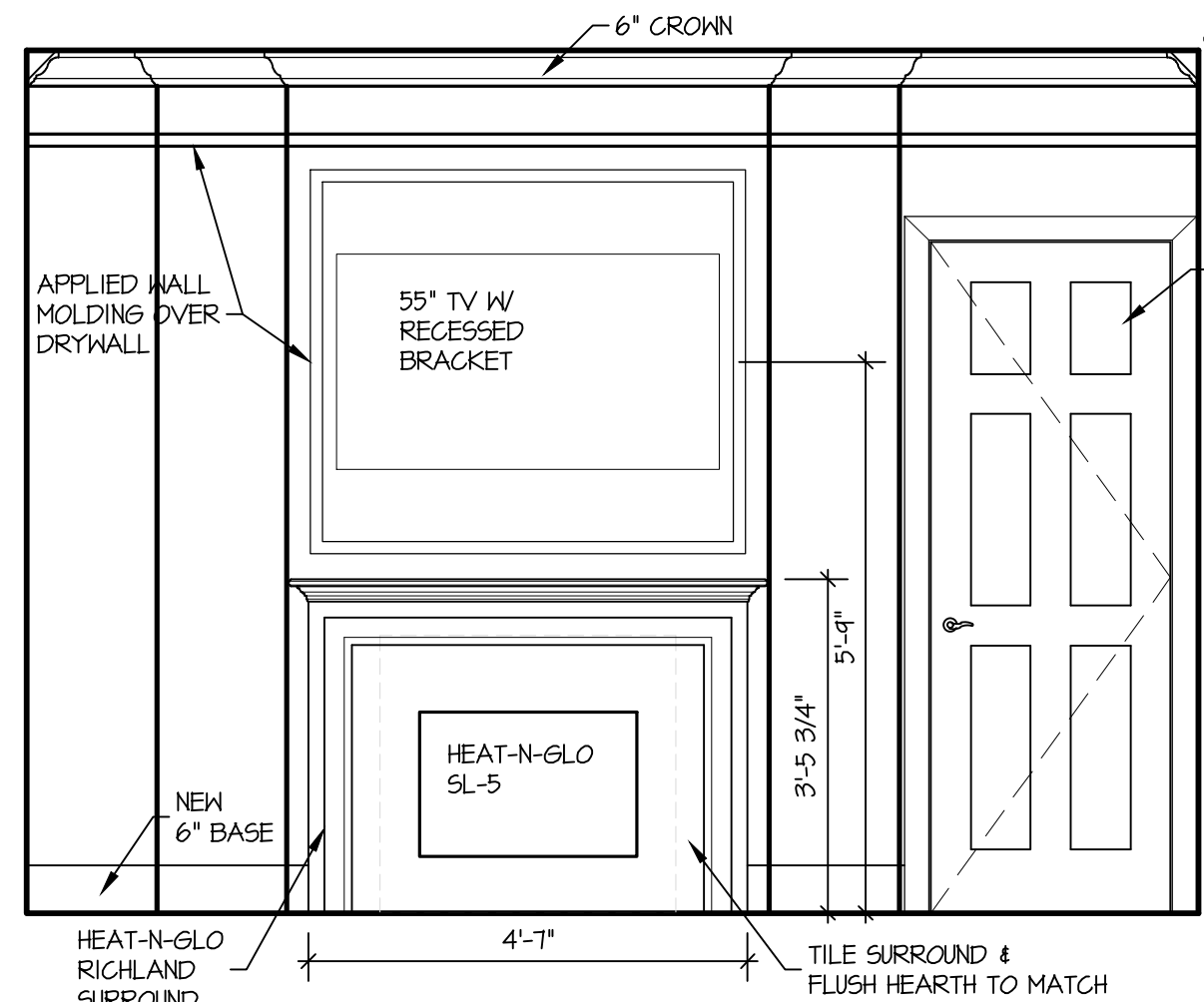
01 PRIMARY BEDROOM 1/2\"/>
