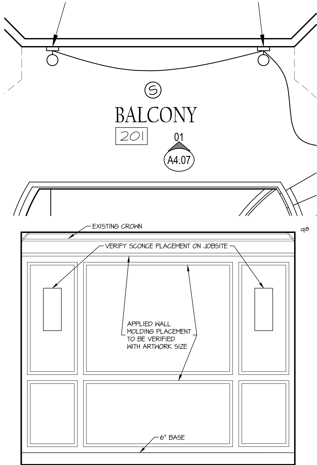
01 BALACONY 1/2" SCALE
