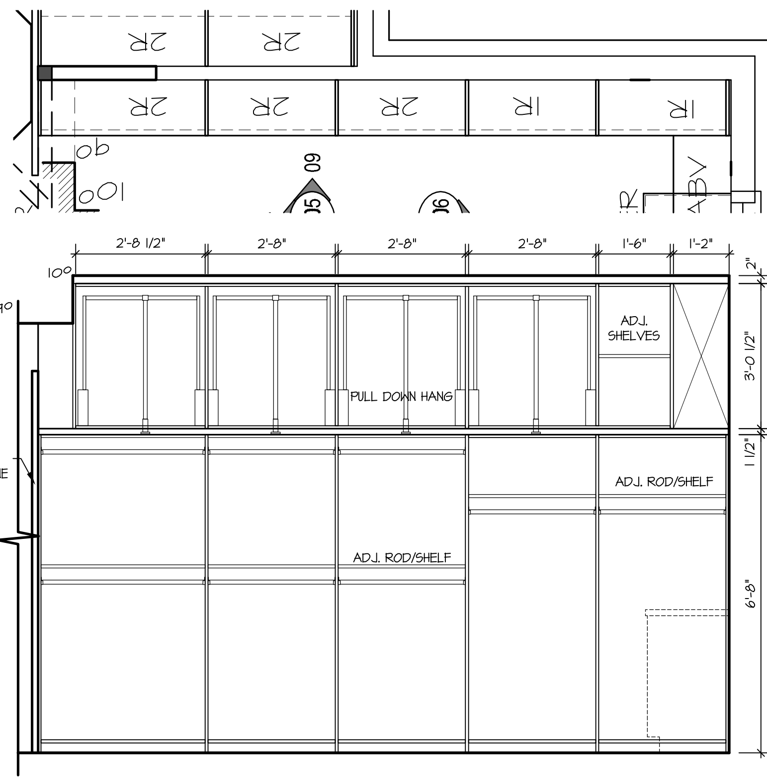
09 PRIMARY WARDROBE 1/2\"/>
