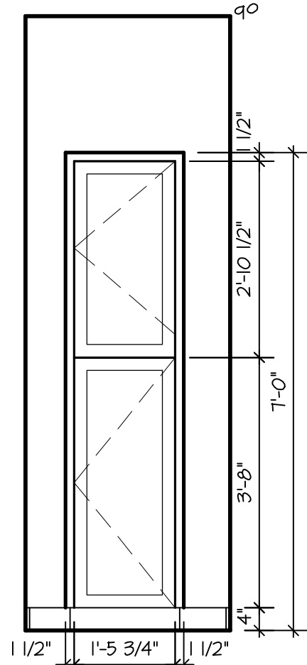
06 PRIMARY BATH 1/2\"/>
