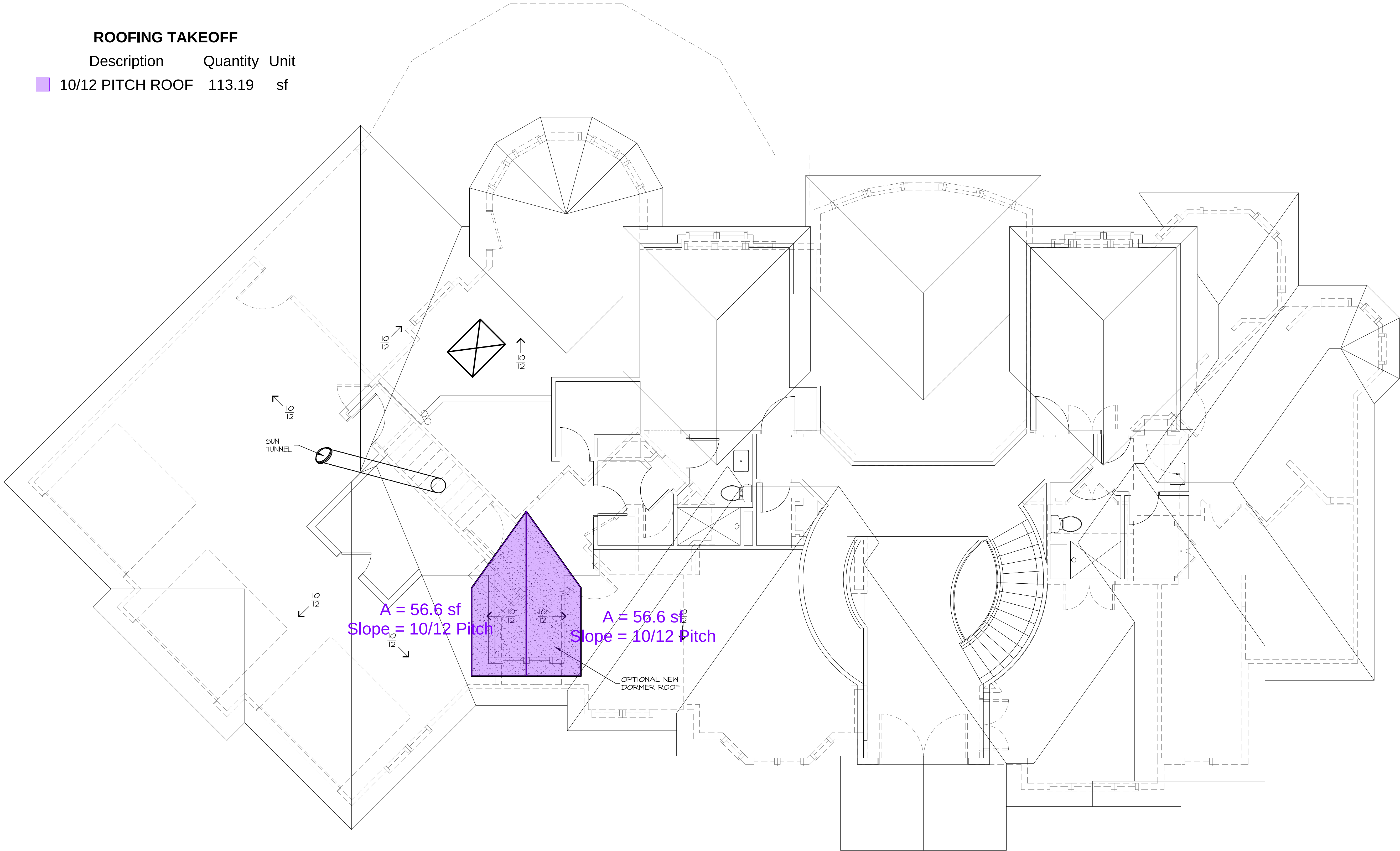
ROOF PLAN
