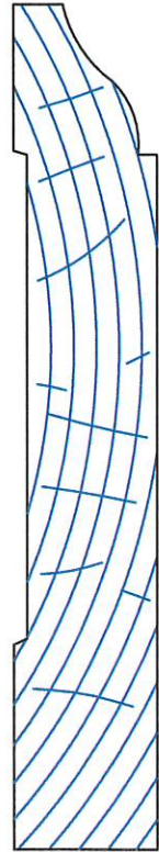
KD 4040 Stock BASE 11/16" x 4"
