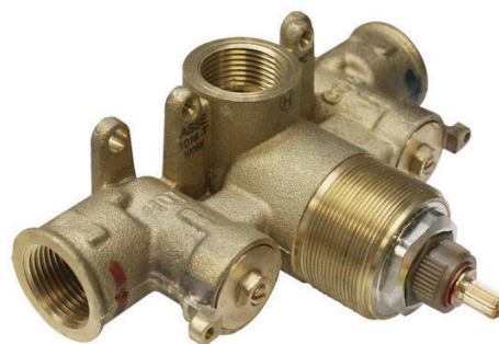
3/4" Thermostatic Rough-In Valve
