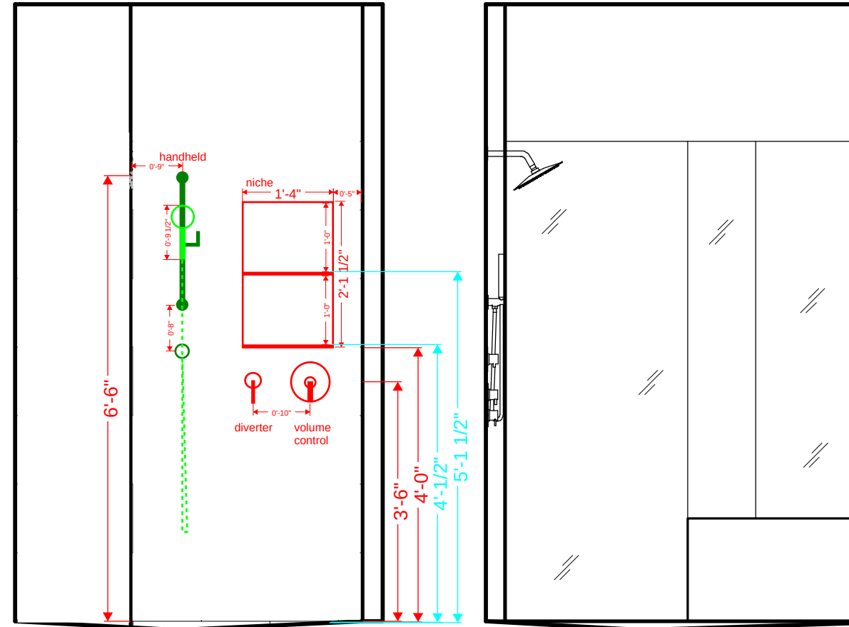
04 PRIMARY SHOWER 1/2" SCALE
