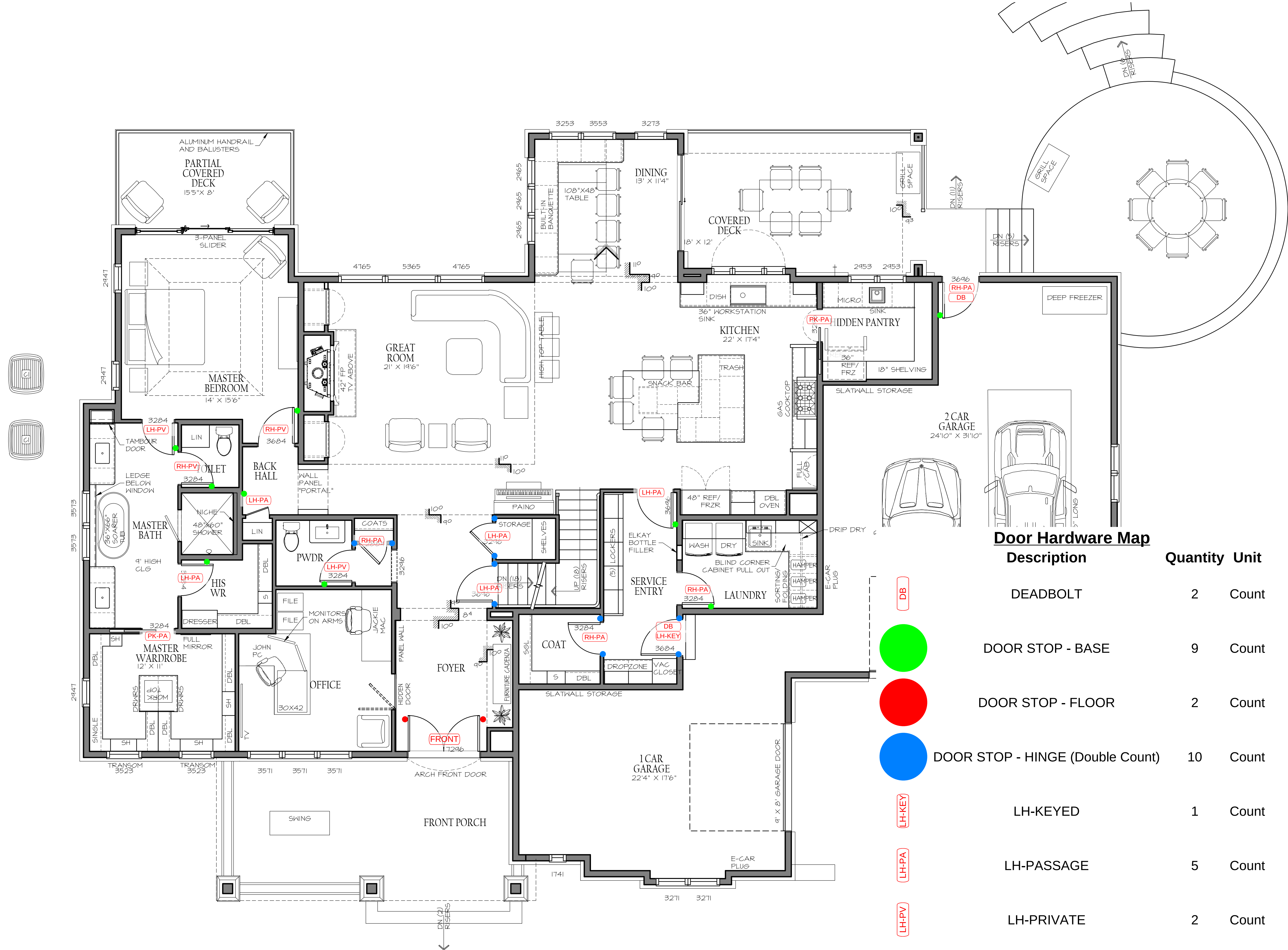
MAIN LEVEL 1/4" = 1'-0"
