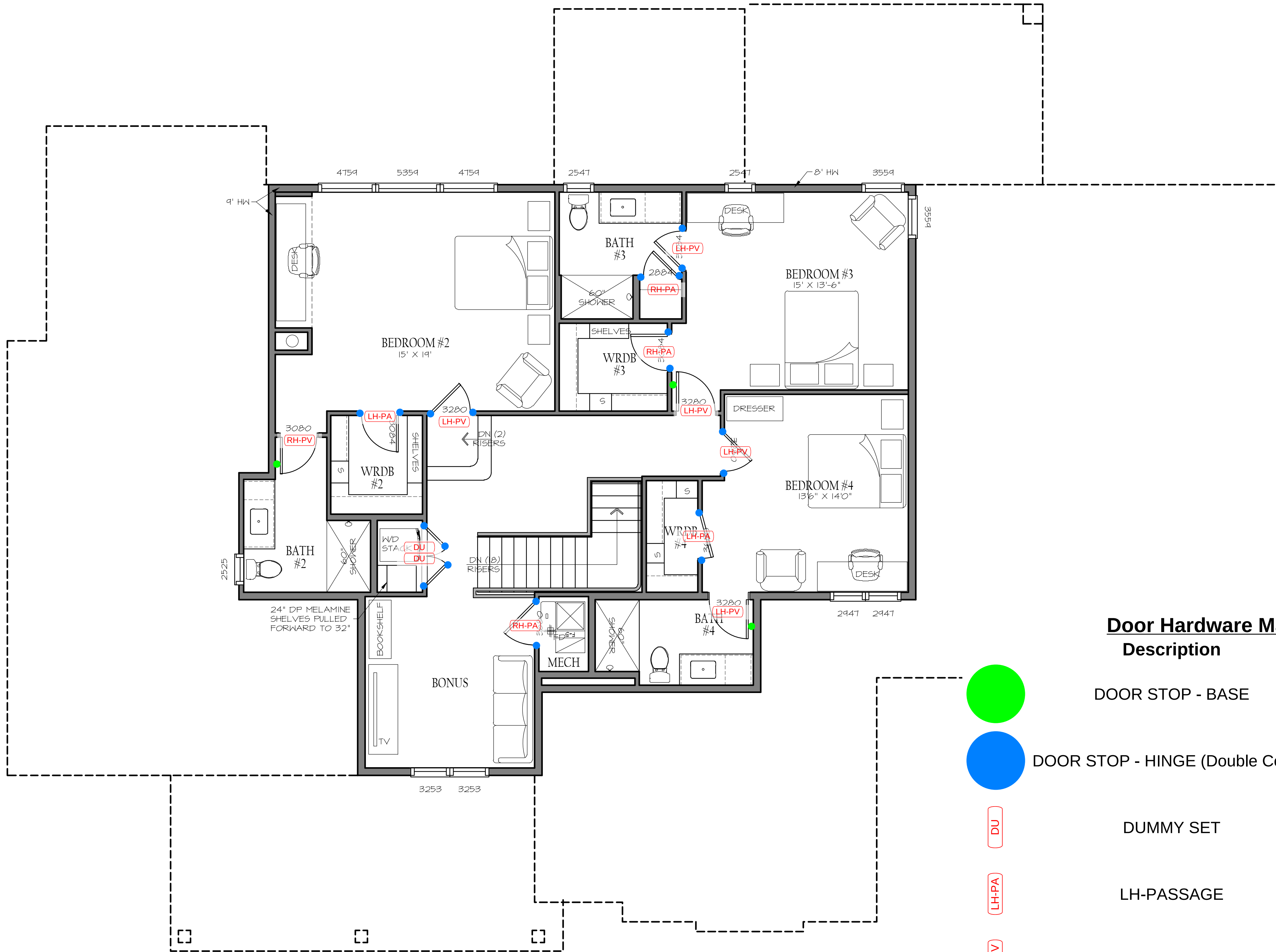
SECOND LEVEL 1/4" = 1'-0"
