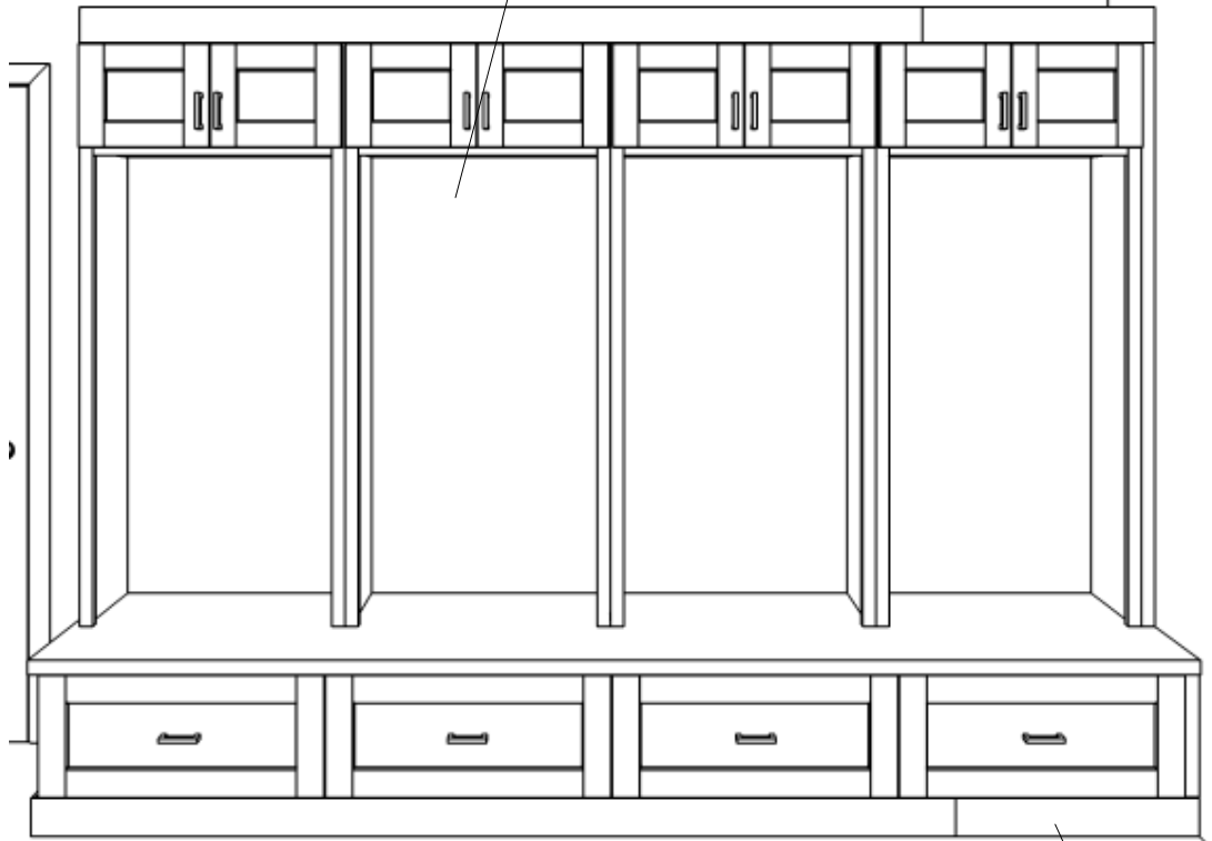
Lockers w/ Finished Interiors
