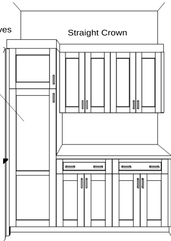
Straight Furniture Base
