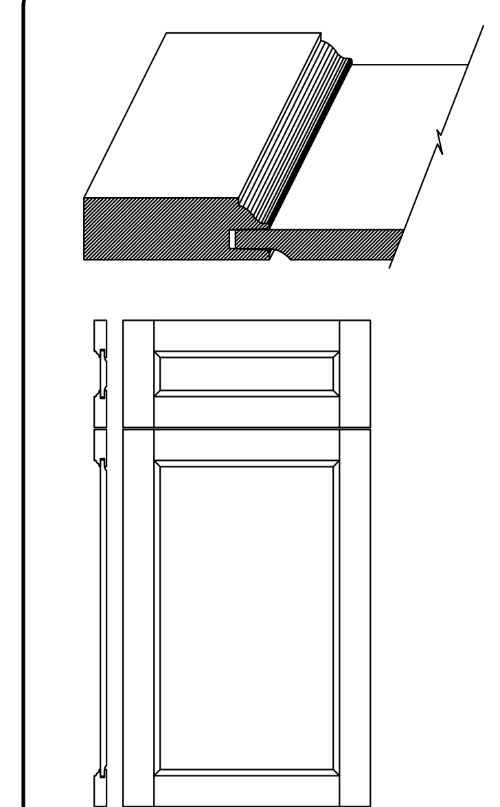
DOOR DETAIL SCALE: 1 1/2" = 1'-0"
