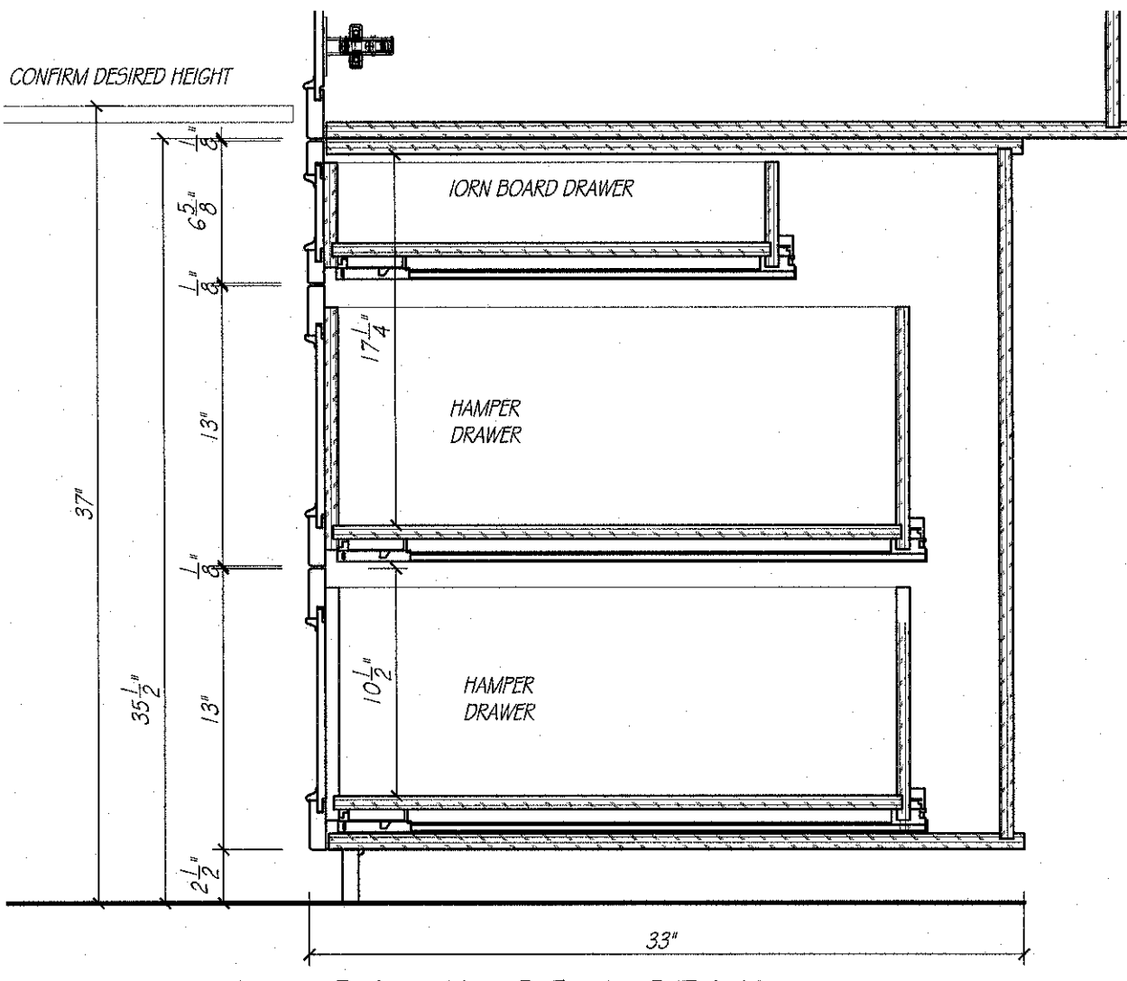
CABINET DETAIL SCALE: 1 1/2" = 1'-0"
