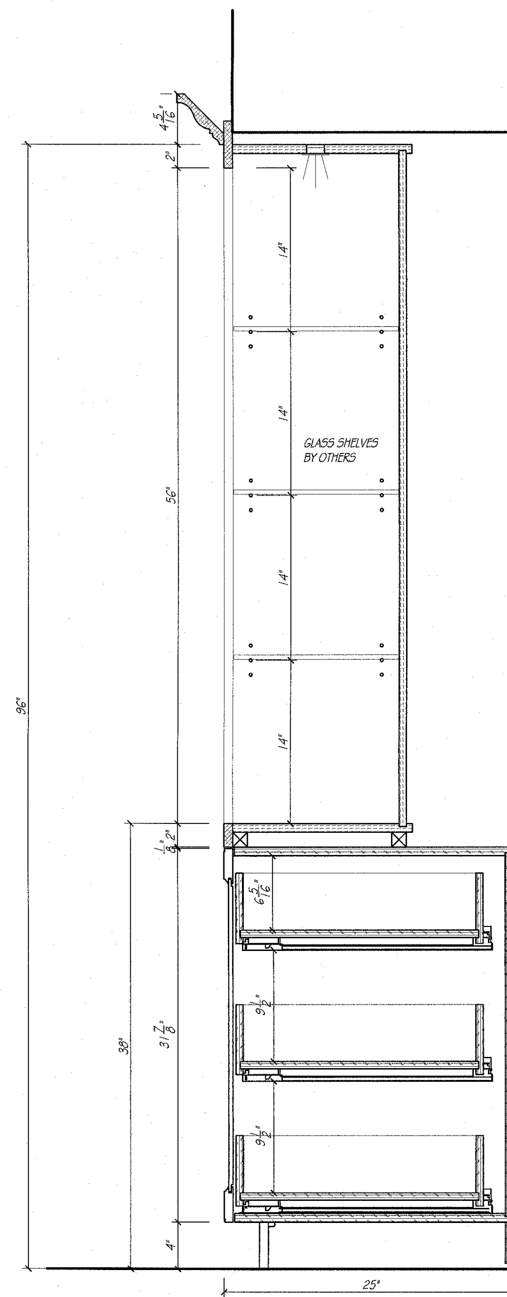
CABINET DETAIL
