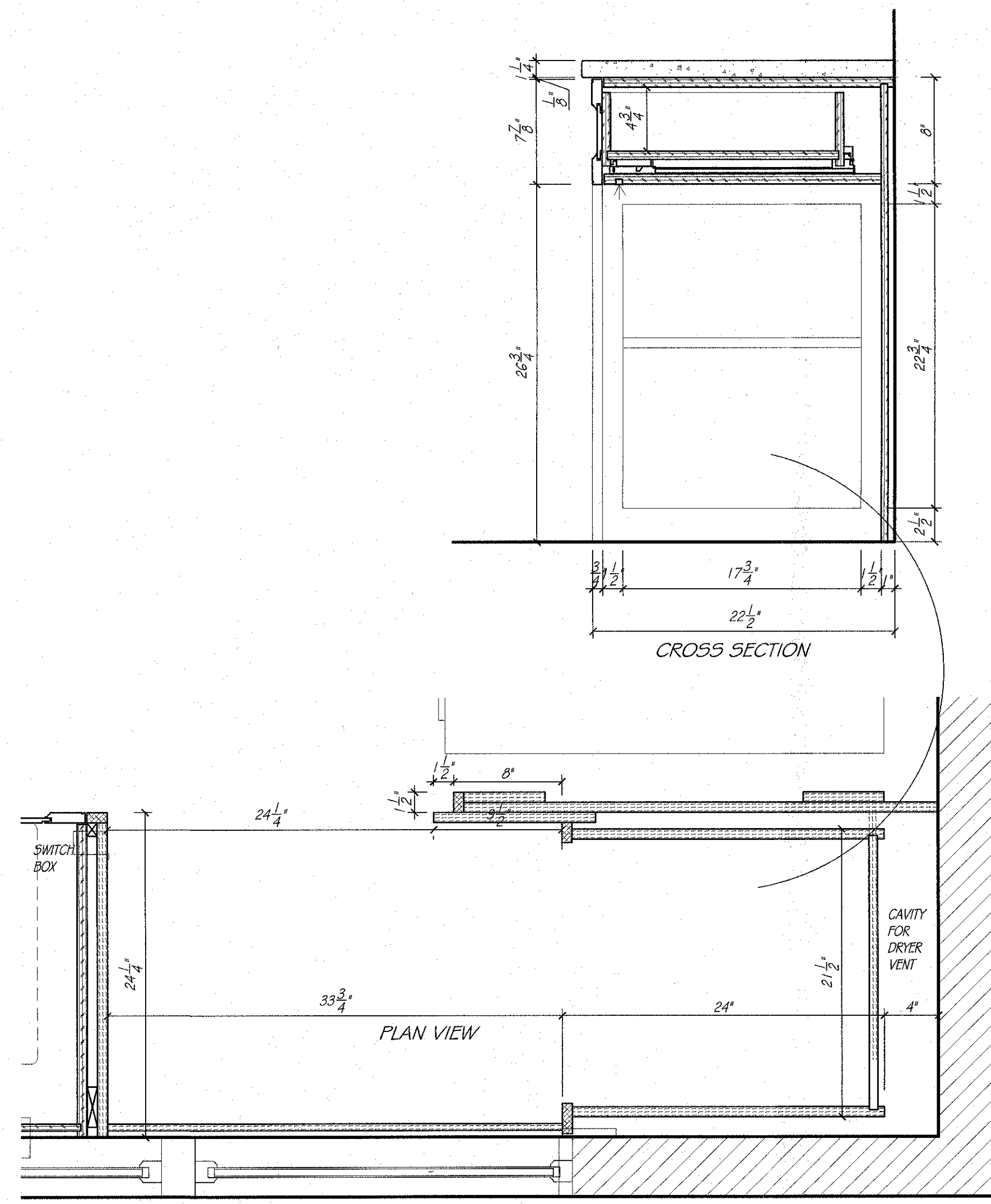
CABINET DETAIL SCALE: 1 1/2" = 1'-0"
