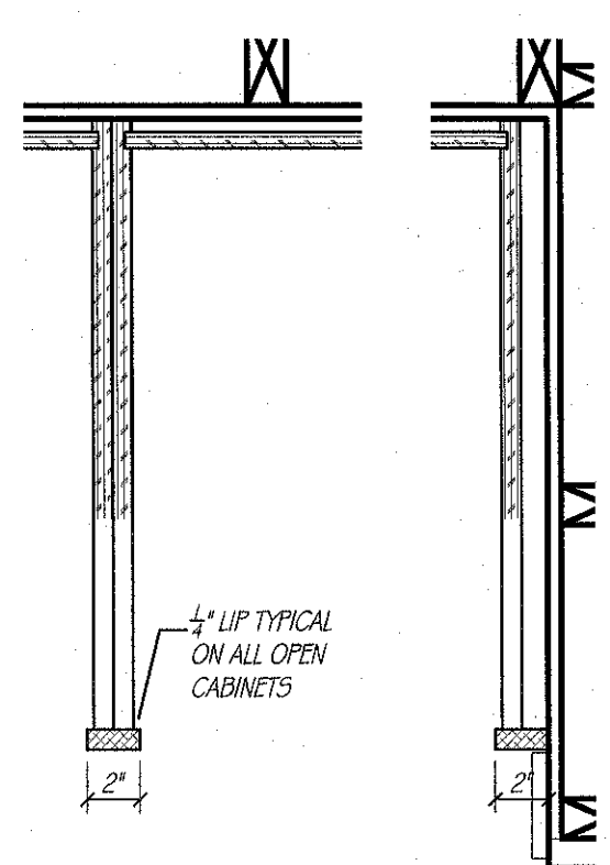
CABINET DETAIL SCALE: 1 1/2" = 1'-0"
