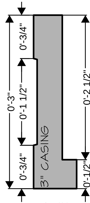
CASING 3/4 x 3
