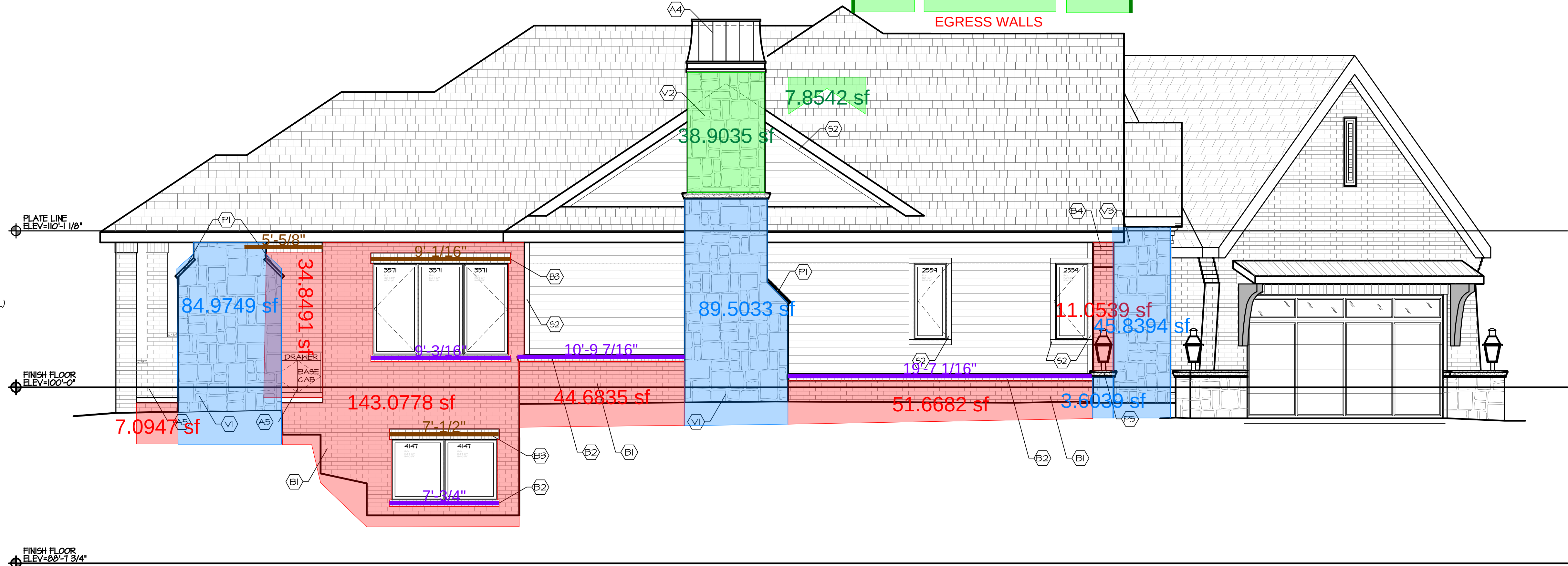
LEFT ELEVATION 1/4"=1'-0"
