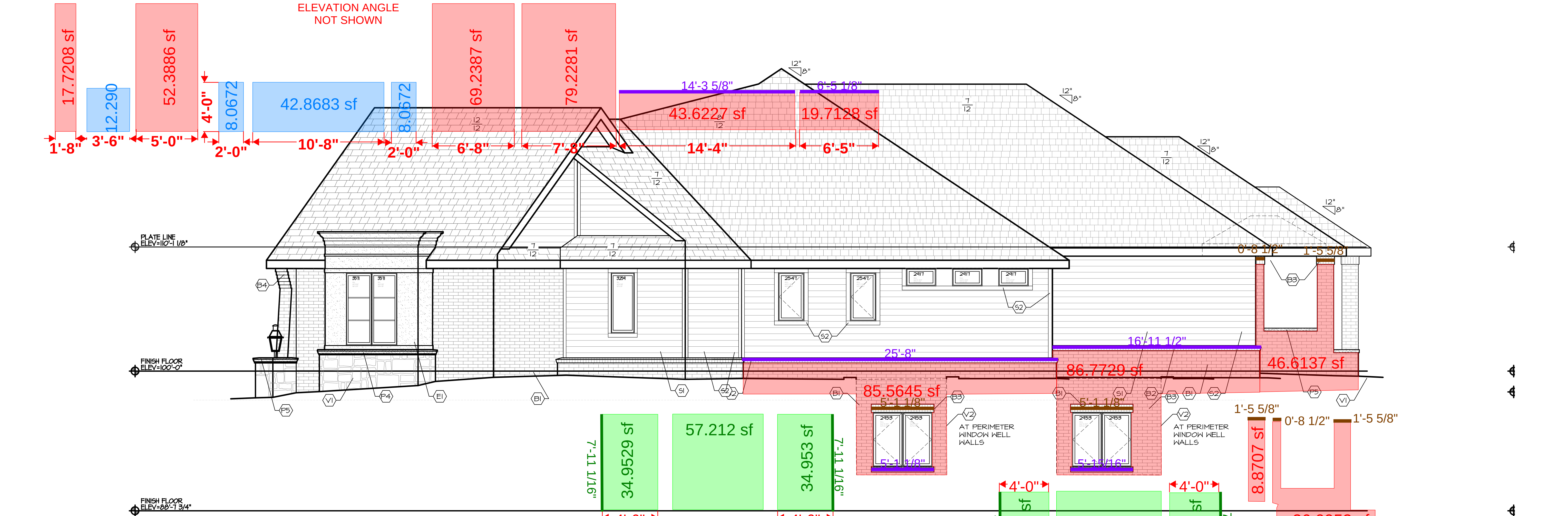
EGRESS WALLS RIGHT ELEVATION 1/4"=1'-0"
