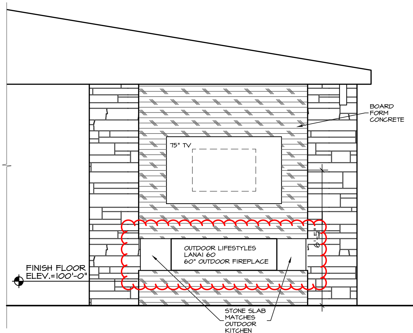
02 OUTDOOR FIREPLACE 3/8" SCALE
