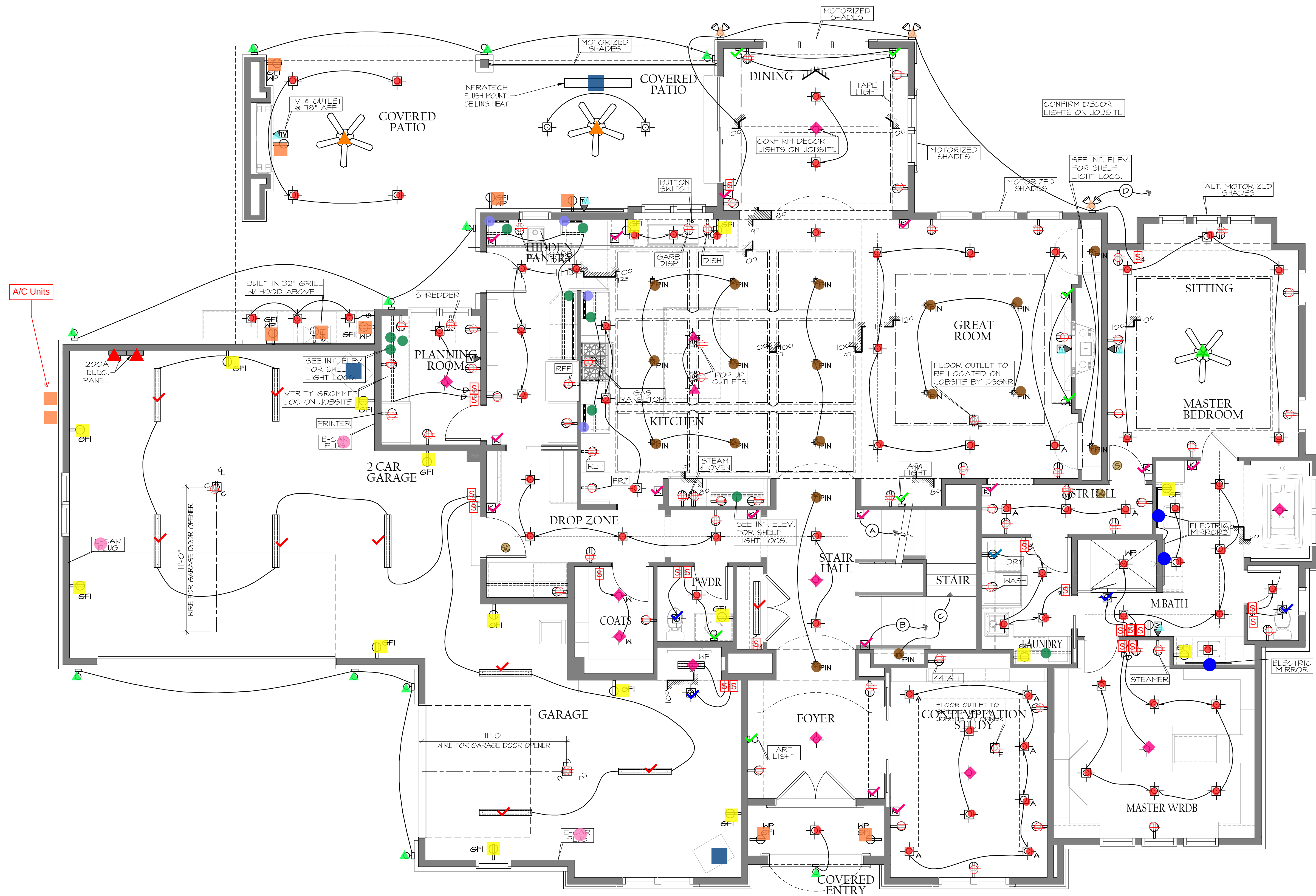
ELECTICAL MAIN LEVEL
