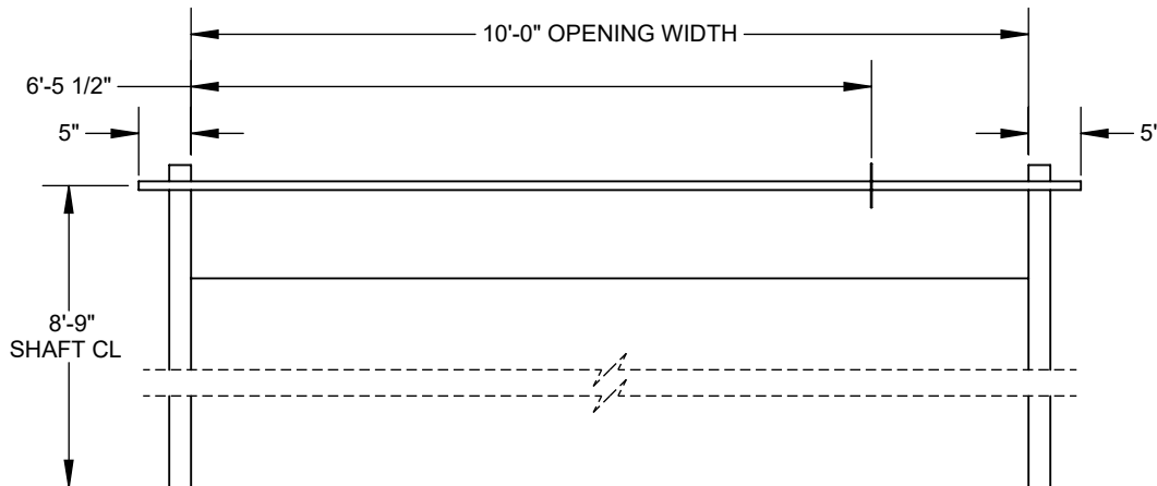
INTERIOR ELEVATION
