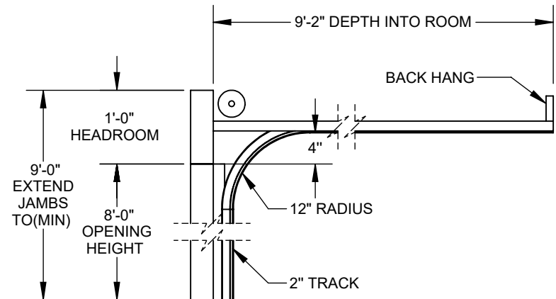
TRACK DETAIL
