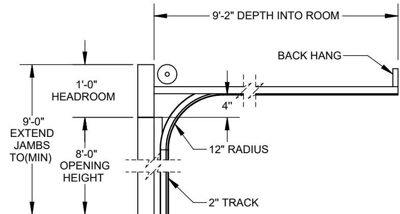
TRACK DETAIL
