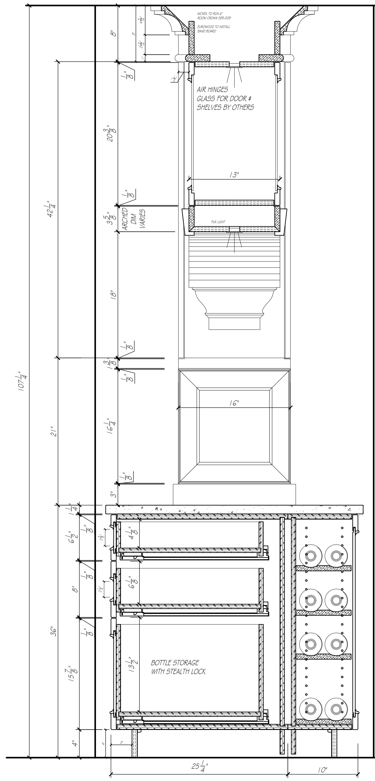
CABINET DETAIL
