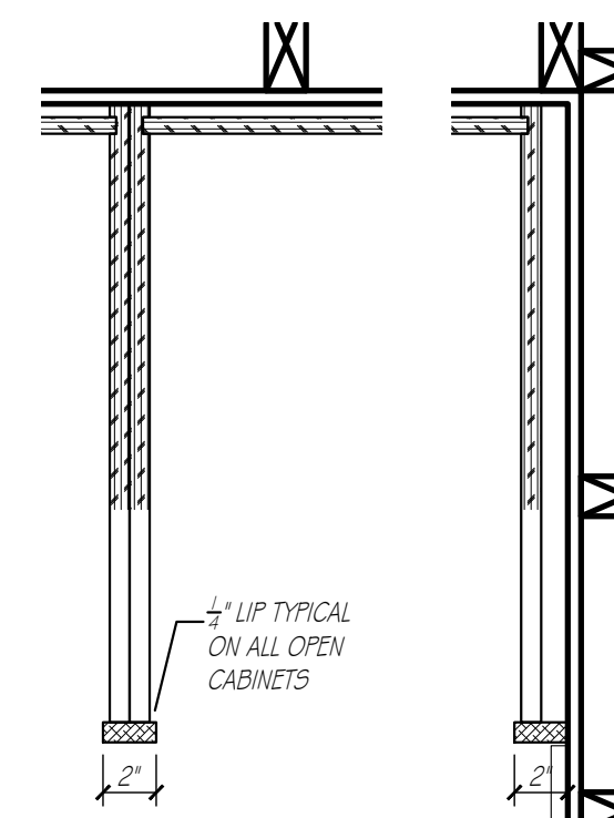
CABINET DETAIL SCALE: 1 1/2" = 1'-0"
