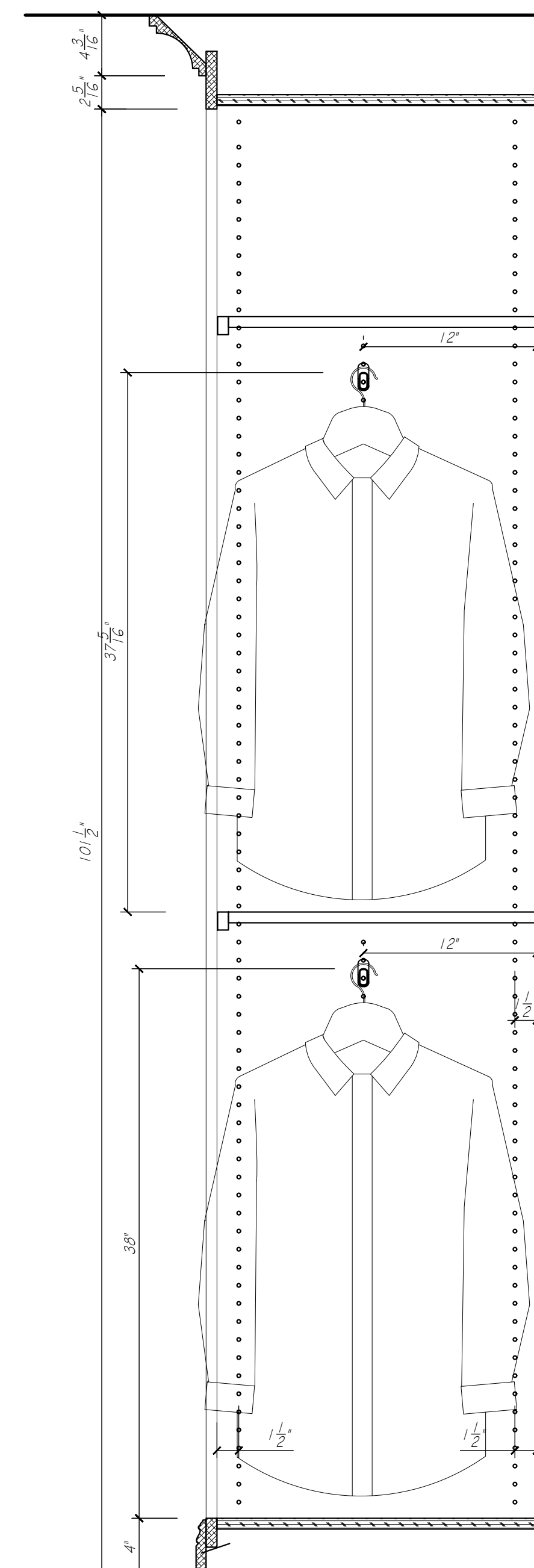
10 A/I CABINET DETAIL SCALE: 1 1/2" = 1'-0"
