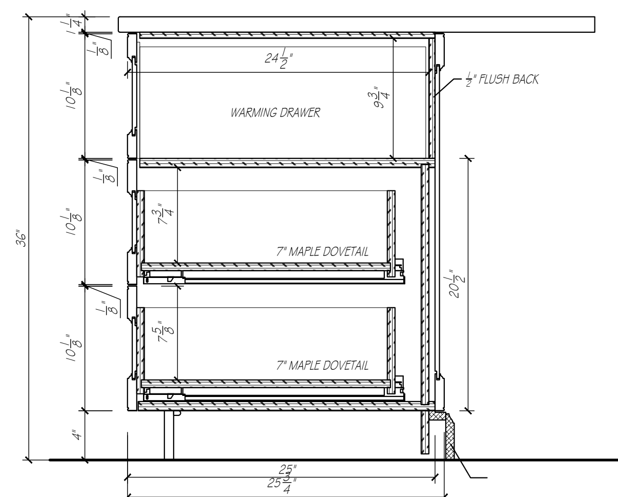
WD CABINET DETAIL SCALE: 1 1/2" = 1'-0"
