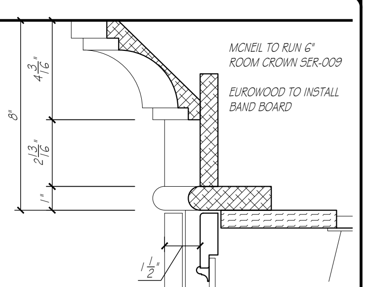
CROWN DETAIL
