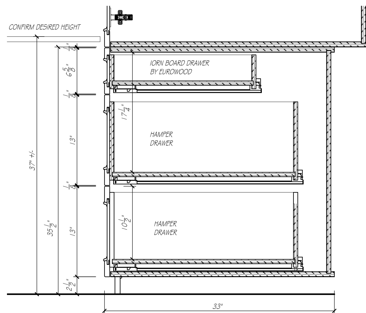
CABINET DETAIL SCALE: 1 1/2" = 1'-0"
