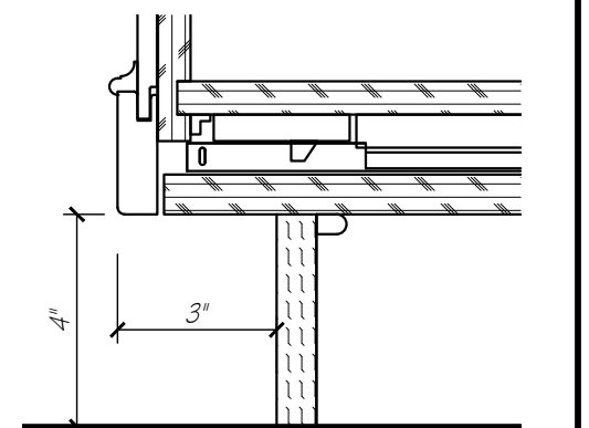
TOE DETAIL
