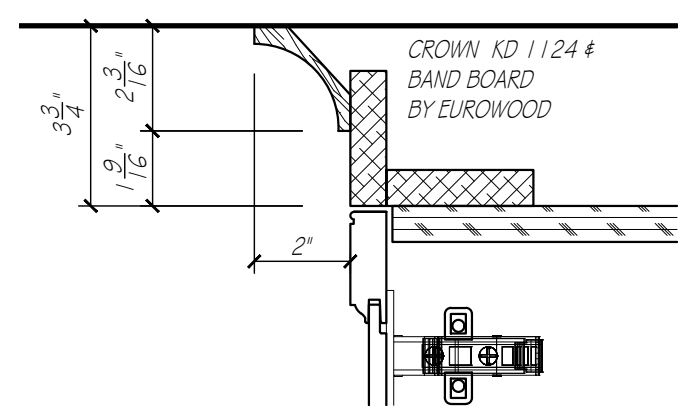
CROWN DETAIL
