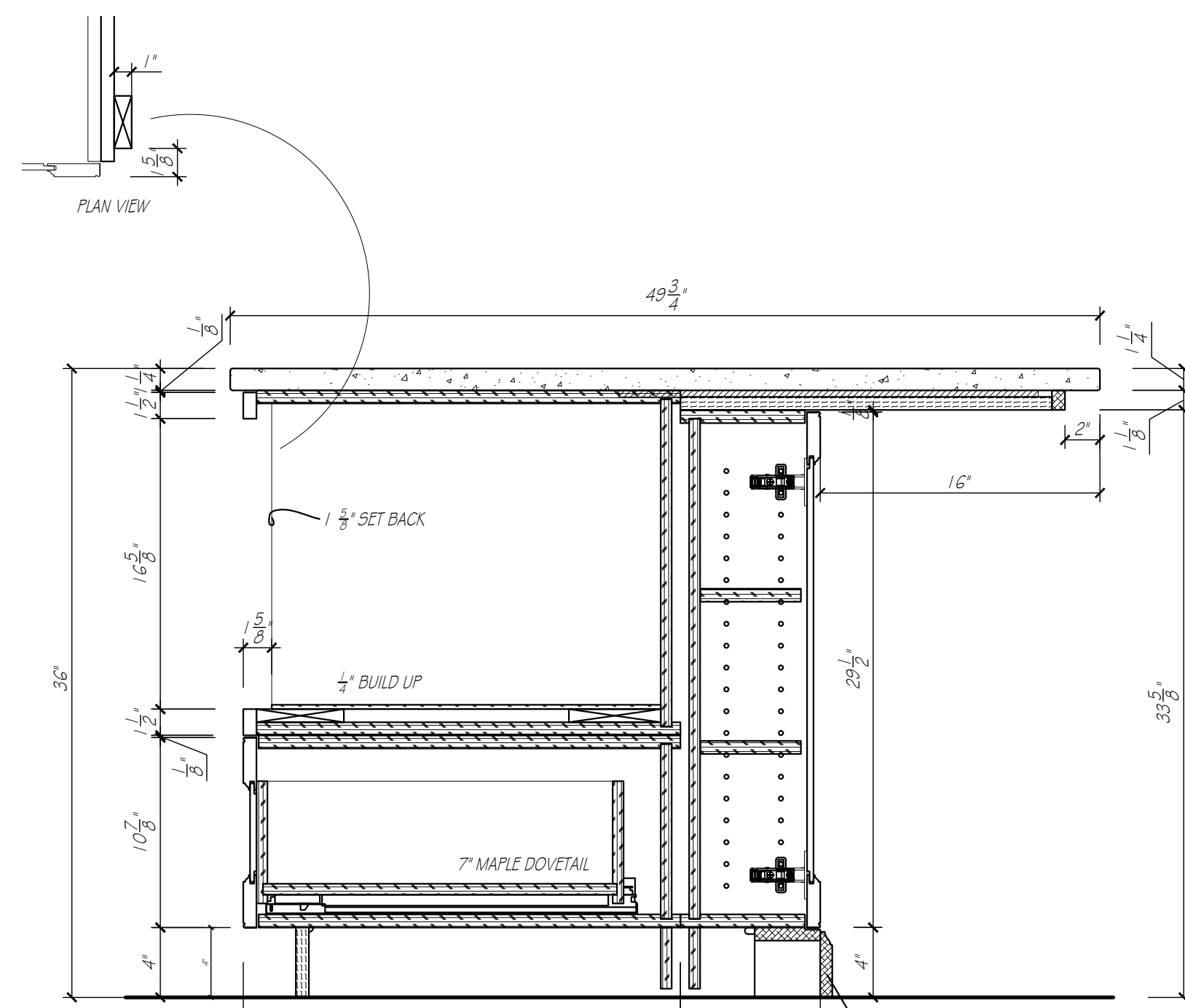
MICROWAVE DRAWER DTL. SCALE: 1 1/2" = 1'-0"
