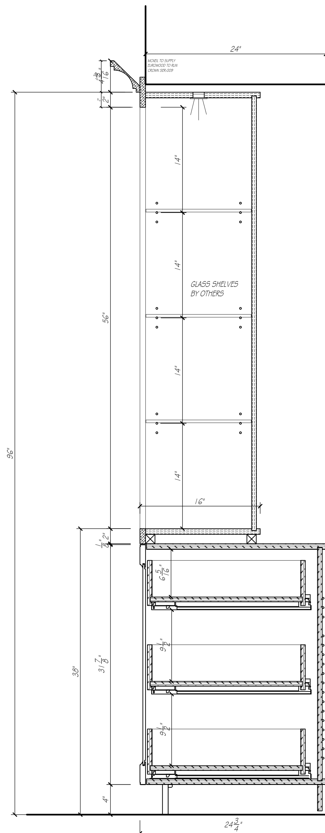
CABINET DETAIL
