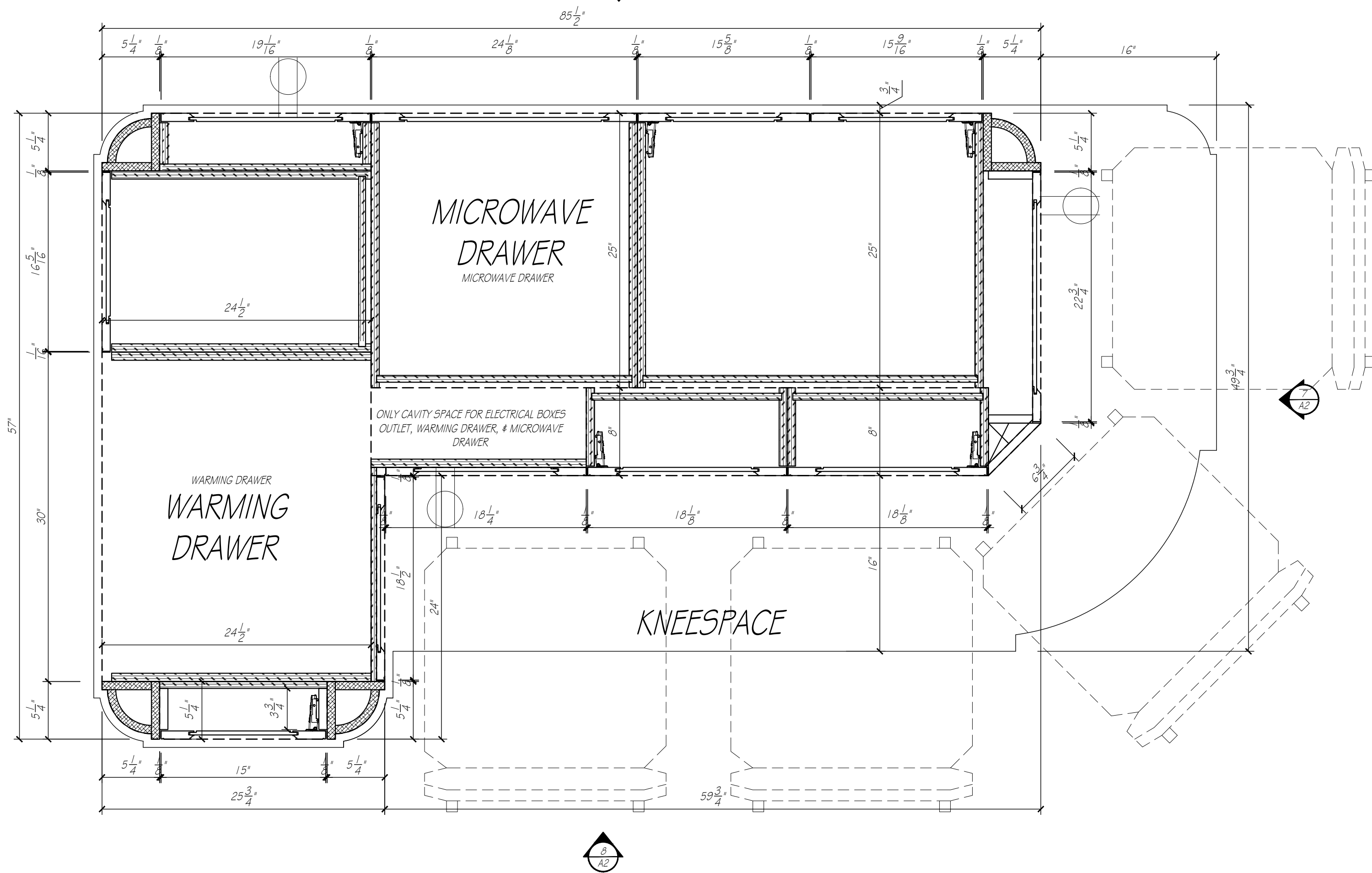
KITCHEN ISLAND SCALE: 1 1/2" = 1'-0"
