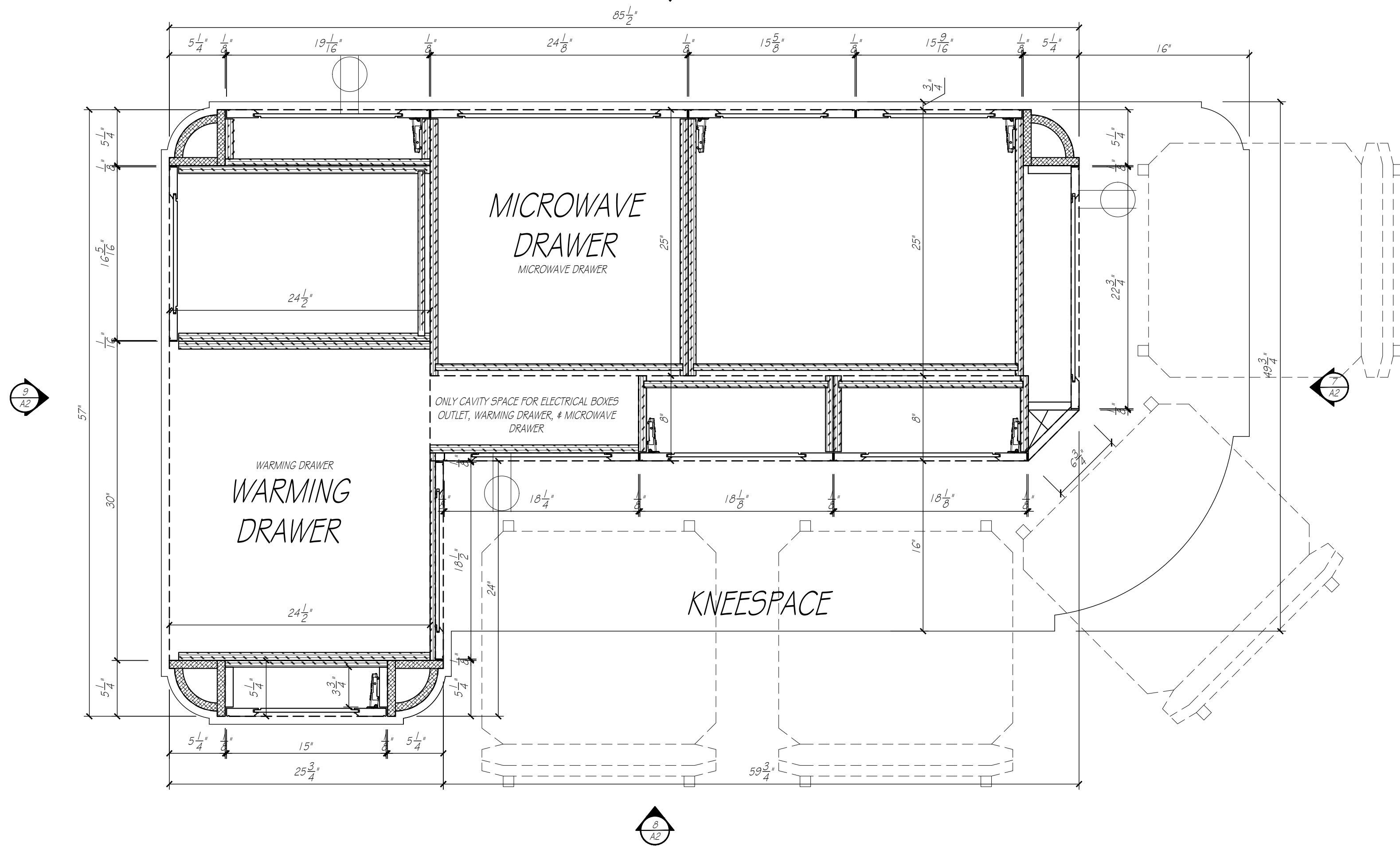
KITCHEN ISLAND SCALE: 1 1/2" = 1'-0"
