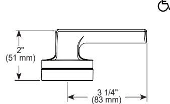
HL6667-GLL Twist Lever Handle - Allaria®
