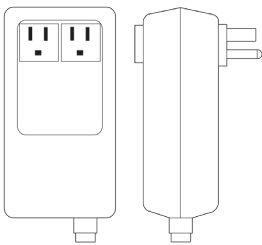
Appliance Control Box 4 3/8"H x 3"W x 1 3/4"D 120v 15Amp 1Hp
