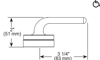
HL6667-GLL Twist Lever Handle - Allaria®
