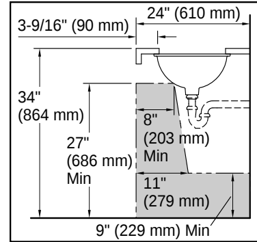
Recommended ADA Installation
