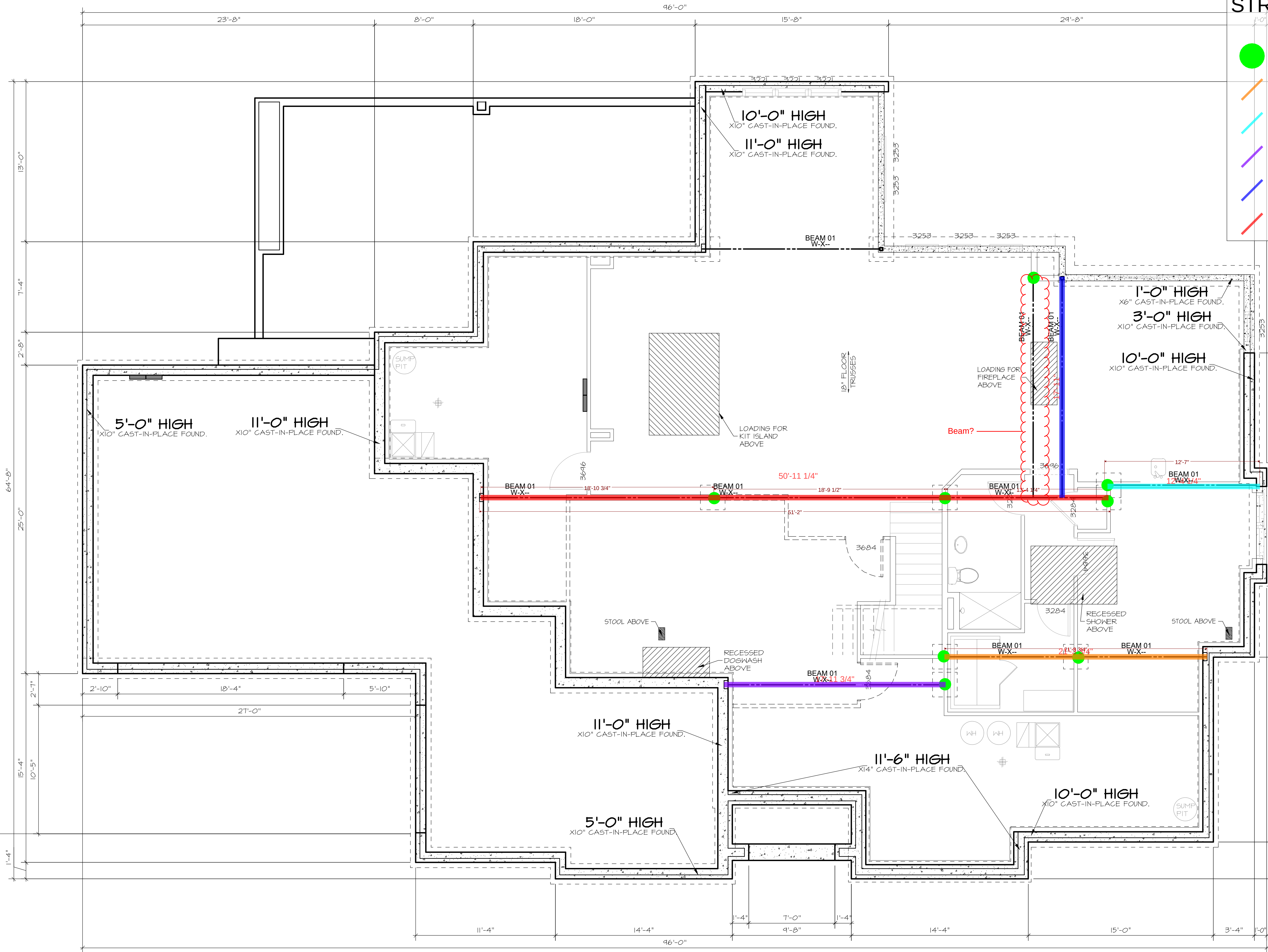
FOUNDATION PLAN
