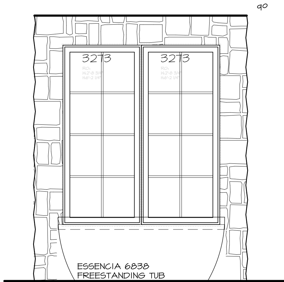
07 TUB 1/2" SCALE
