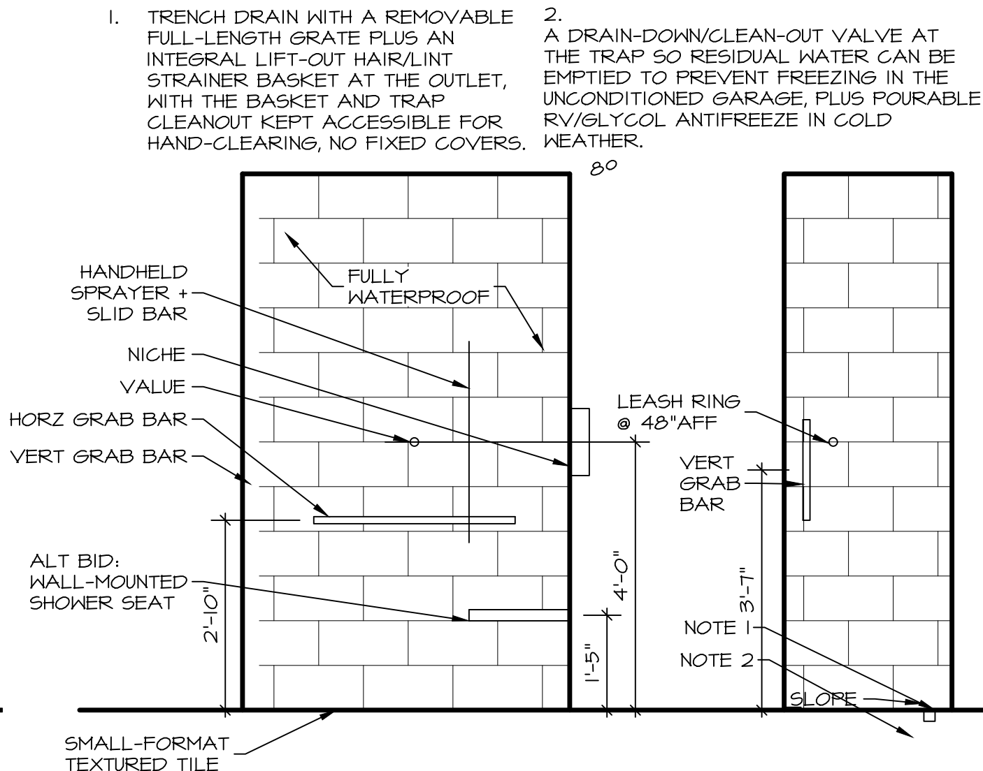
08 DOGWASH 1/2" SCALE
