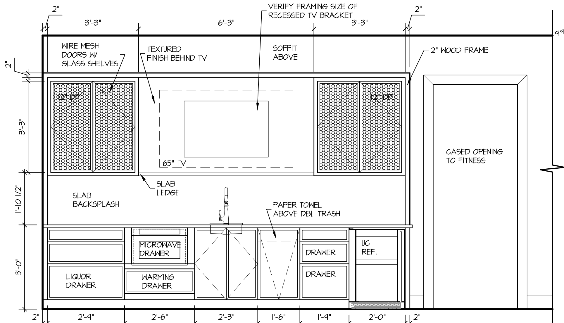
03 BAR 1/2" SCALE
