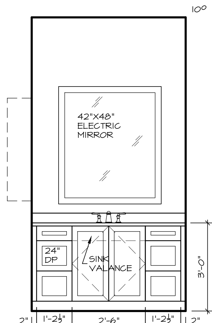
05 HIS VANITY 1/2" SCALE
