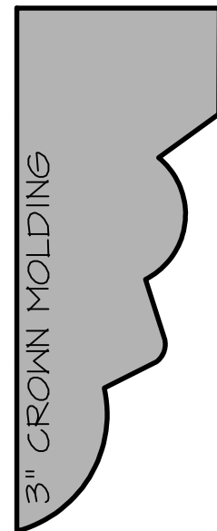
SEA-007 1-3/16 x 3
