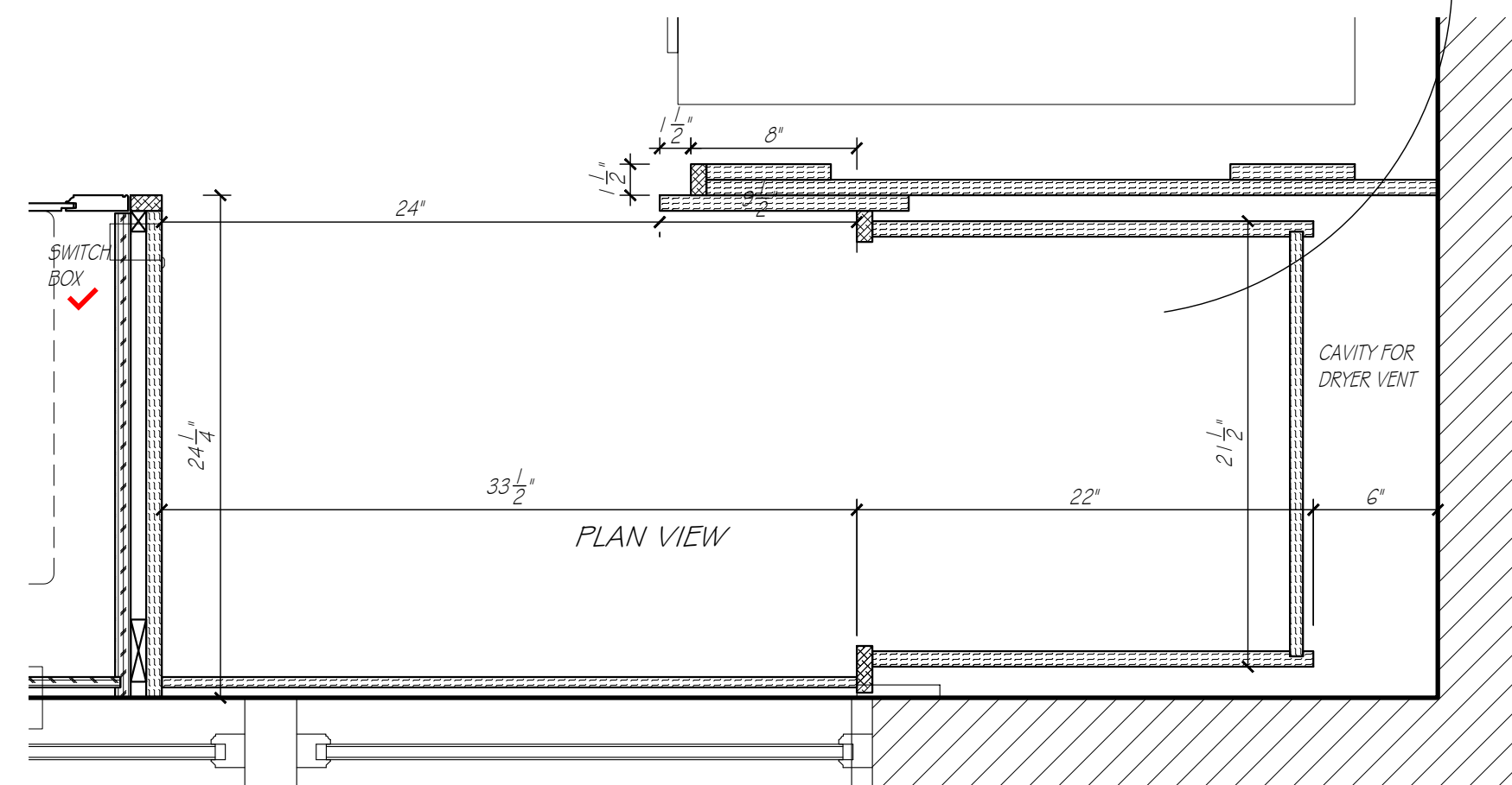
6 CABINET DETAIL SCALE: 1 1/2" = 1'-0"
