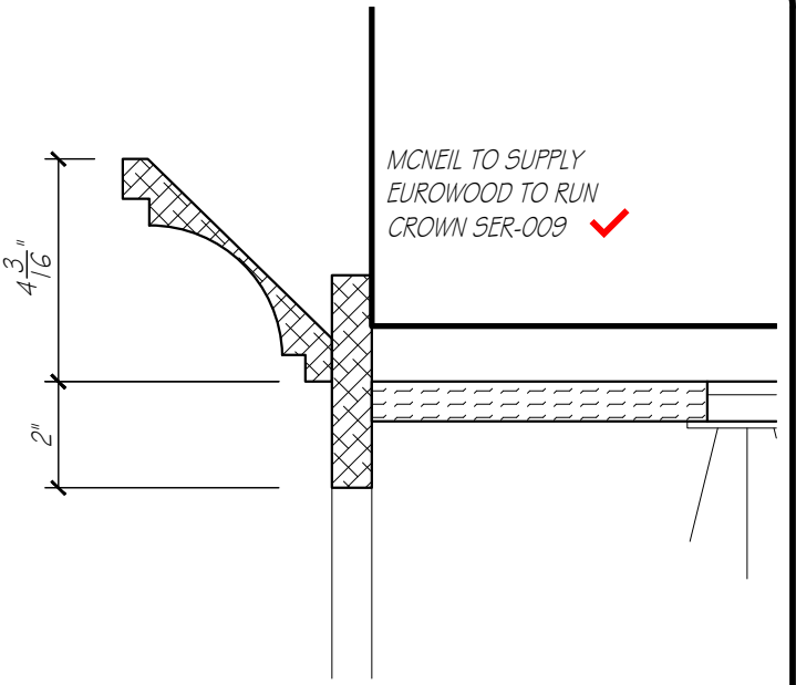
CROWN DETAIL
