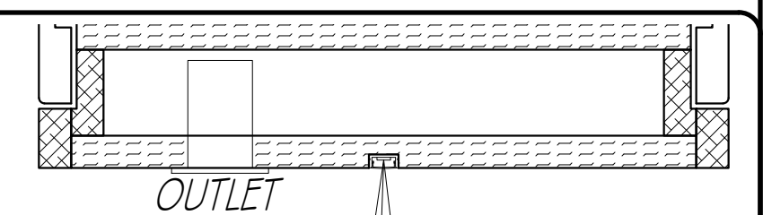
LC DETAIL ✓
