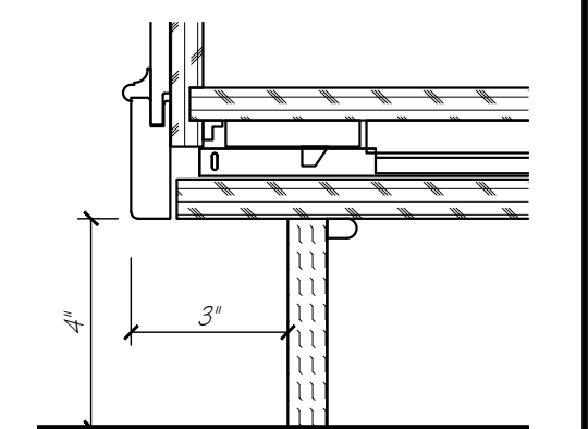
TOE DETAIL ✓
