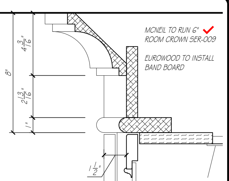
CROWN DETAIL ✓
