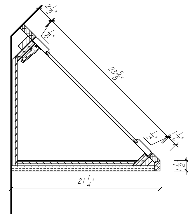
5 BASE CABINET DETAIL SCALE: 1 1/2" = 1'-0"
