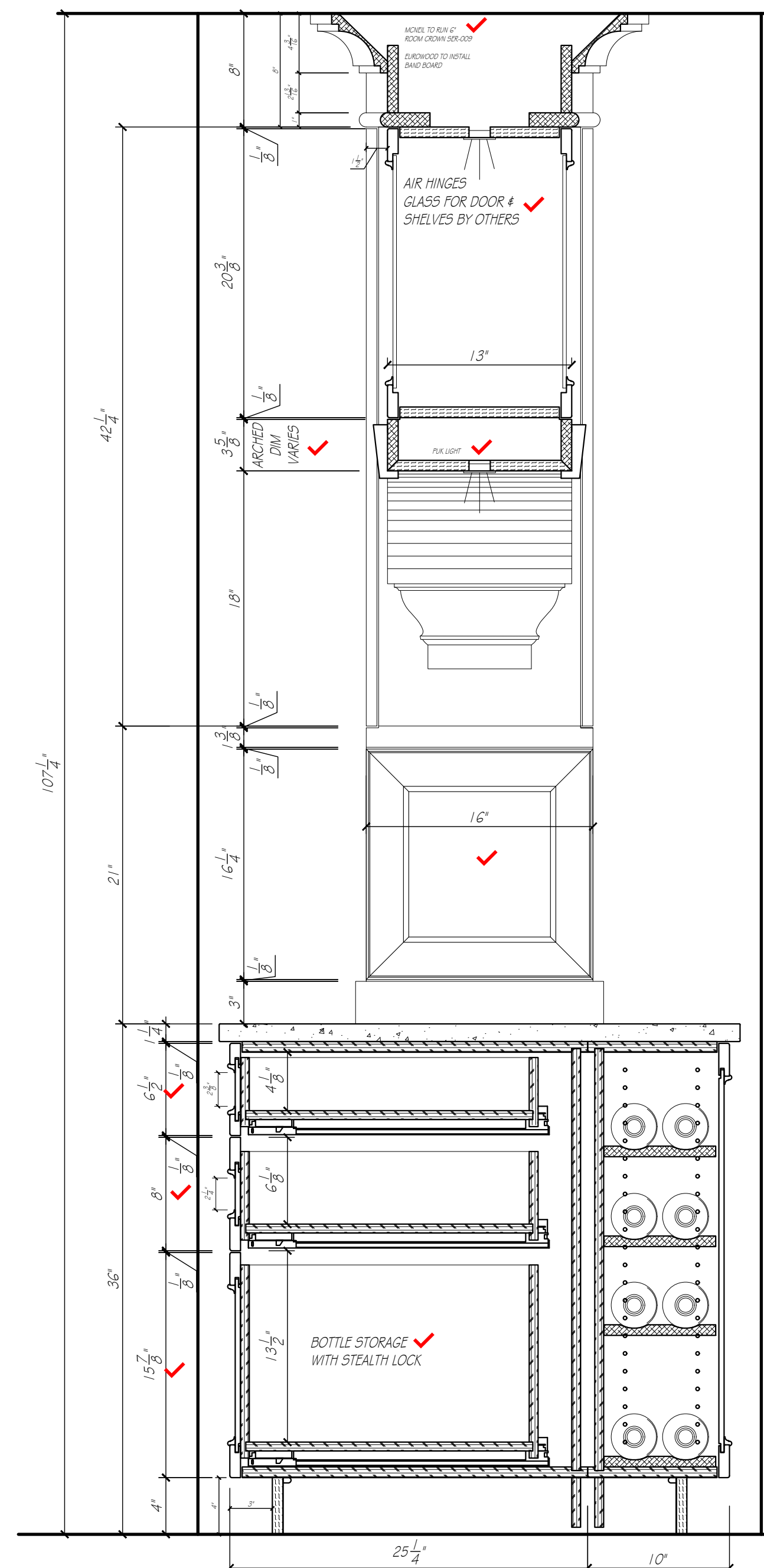
CABINET DETAIL
