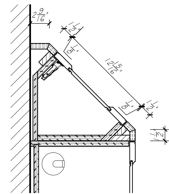
4 UPPER CABINET DETAIL SCALE: 1 1/2" = 1'-0"
