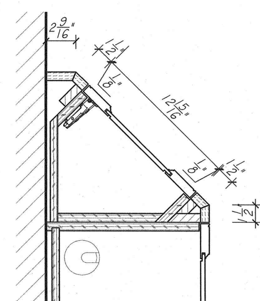
4 UPPER CABINET DETAIL SCALE: 1 1/2" = 1'-0"
