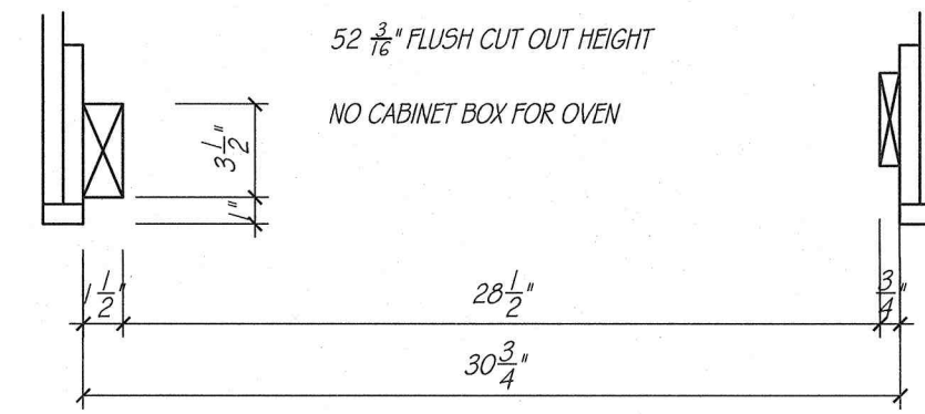
THERMADOR DOUBLE OVEN 30" MODEL-MED302LWS FLUSH INSTALL
