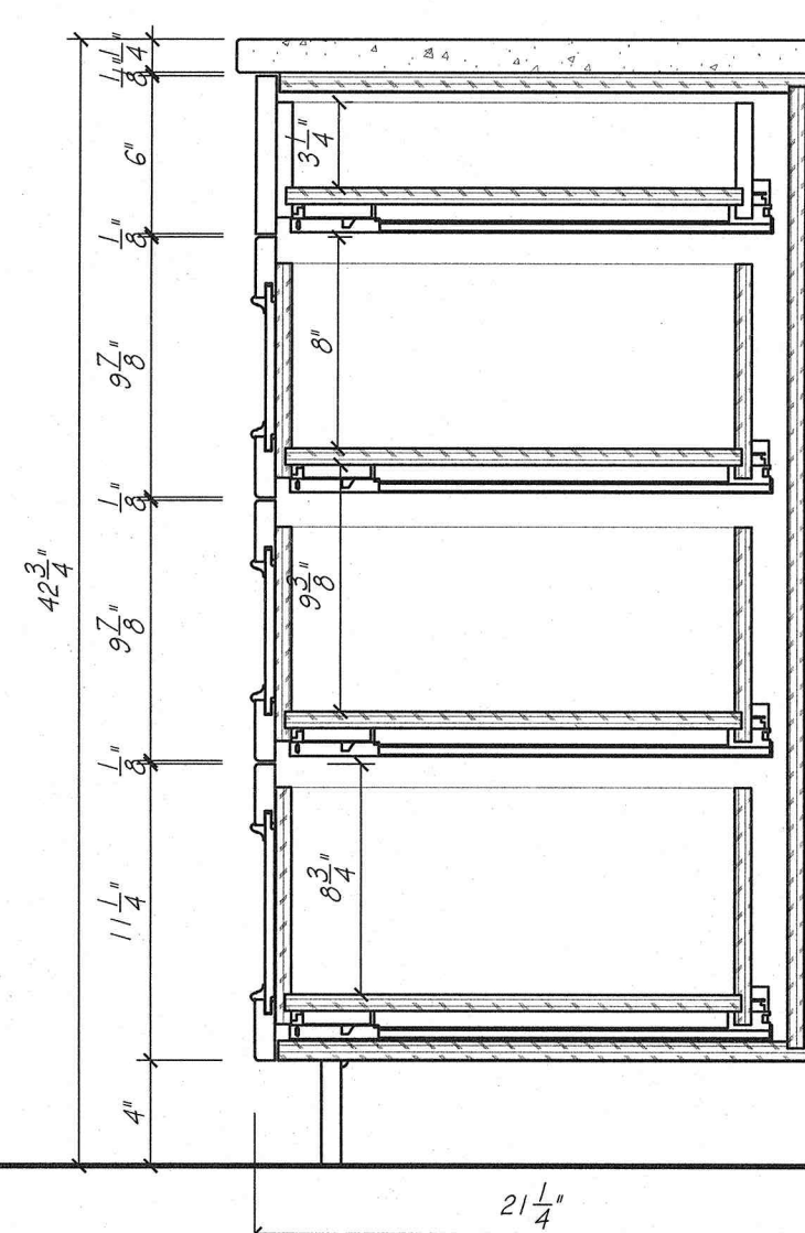
CABINET DETAIL SCALE: 1 1/2" = 1'-0"
