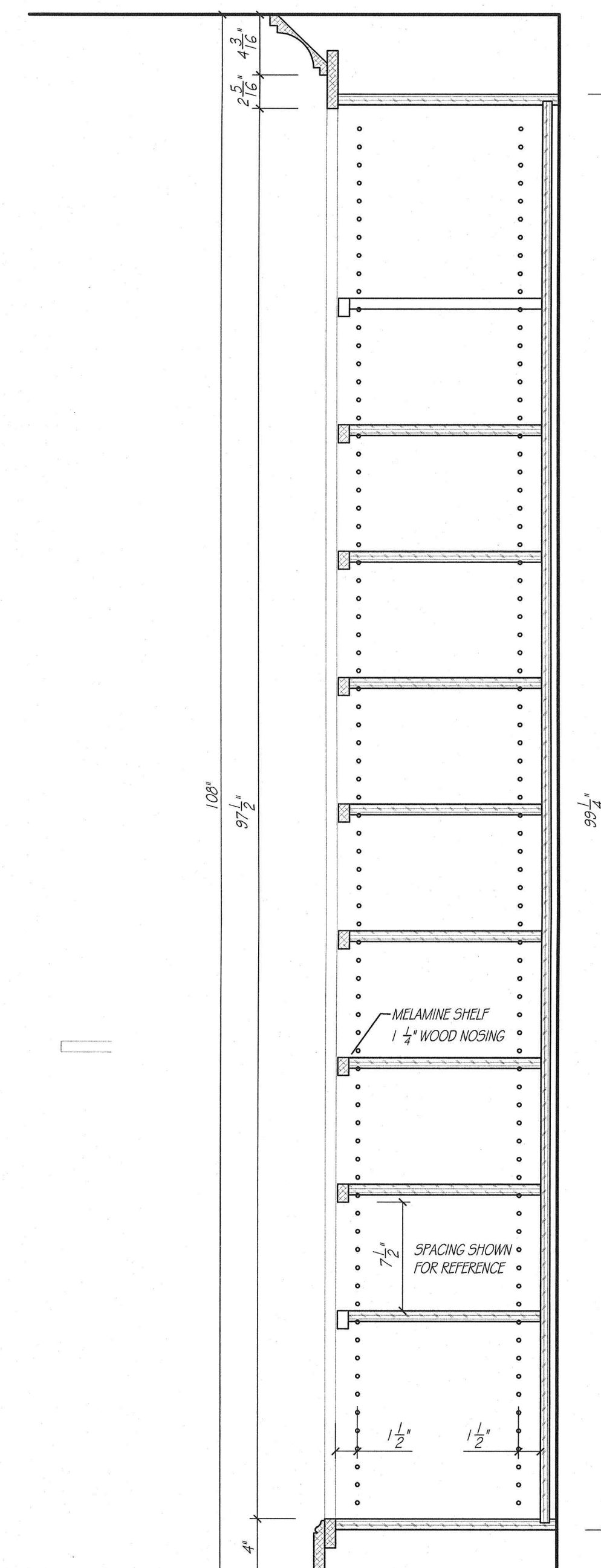
CABINET DETAIL SCALE: 1 1/2" = 1'-0"
