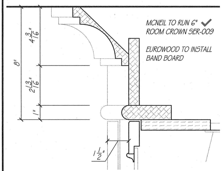
CROWN DETAIL ✓ SCALE: 3" = 1'-0"
