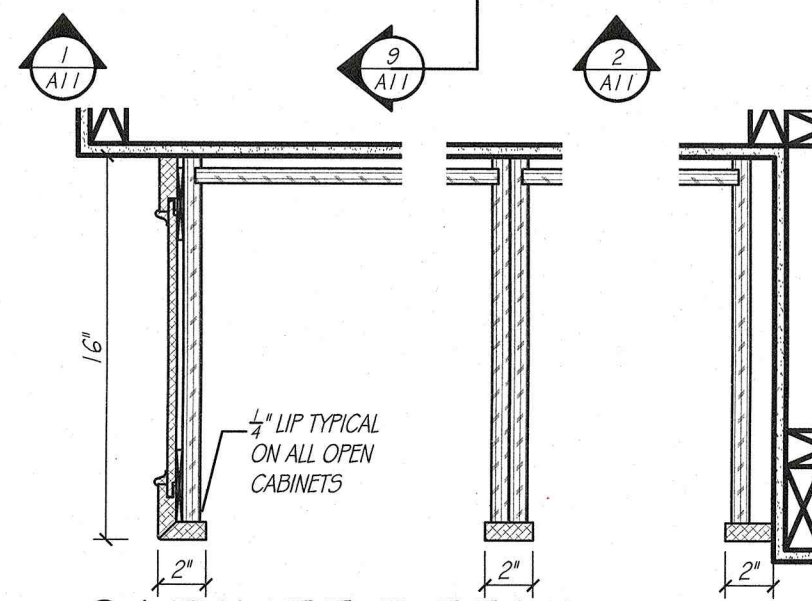
CABINET DETAIL SCALE: 1 1/2" = 1'-0"
