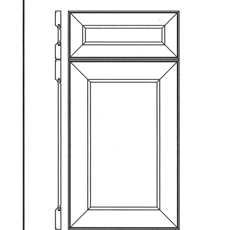
DOOR DETAIL ✓ EW-CWS SCALE: 1 1/2" = 1'-0"
