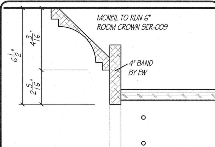
CROWN DETAIL SCALE: 3\"/>
