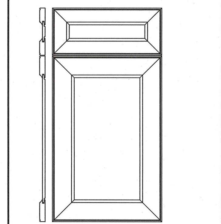
DOOR DETAIL SCALE: 1 1/2" = 1'-0"
