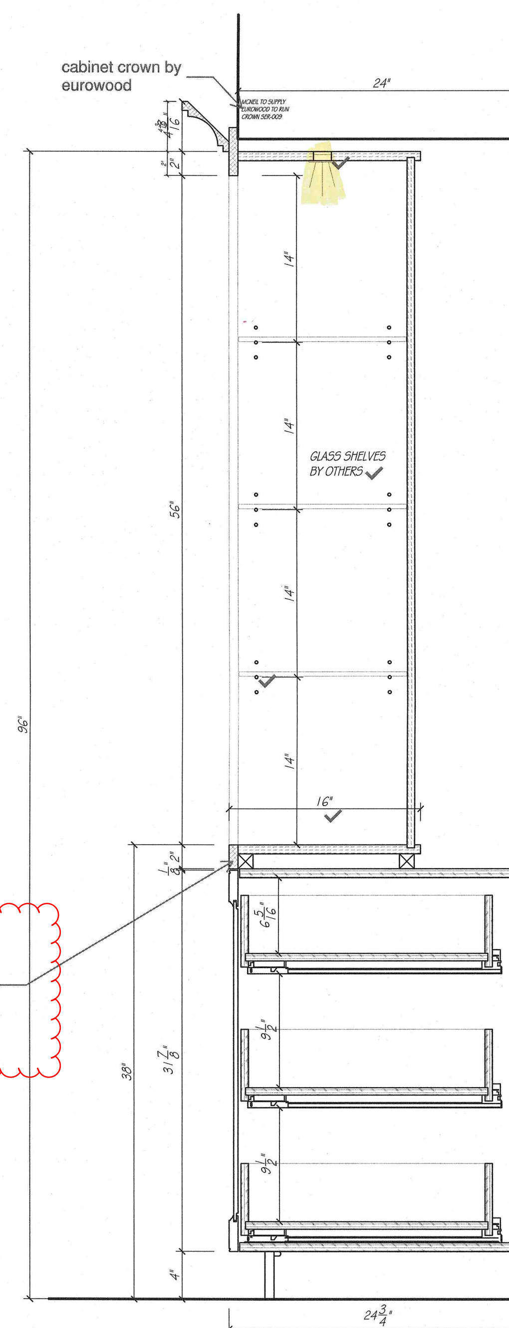
CABINET DETAIL SCALE: 1 1/2" = 1'-0"
