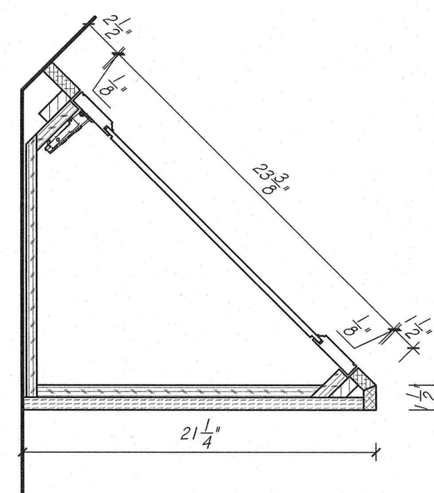
5 BASE CABINET DETAIL SCALE: 1 1/2" = 1'-0"
