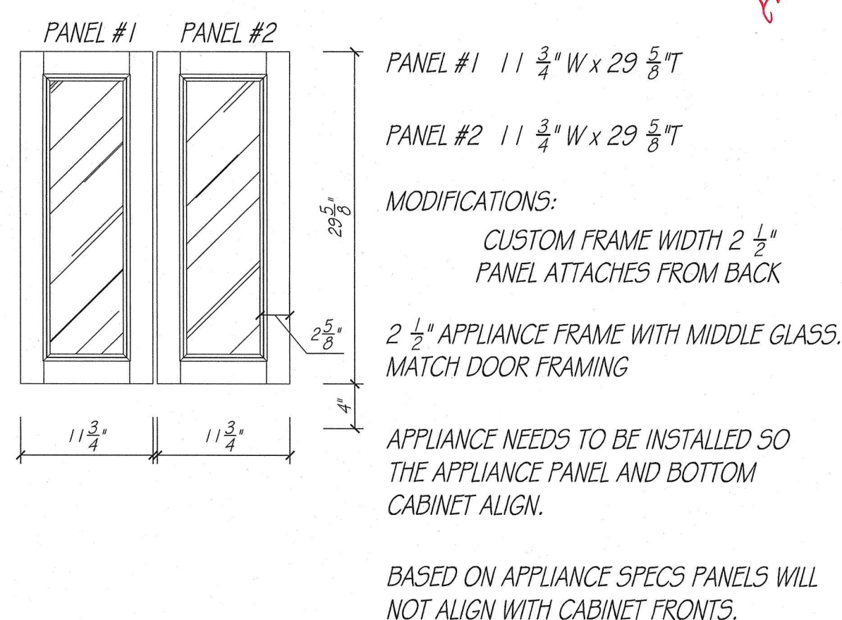
AVALLON BEVERAGE REFRIGERATOR MODEL - AWBC242GGFDPRG ✓
