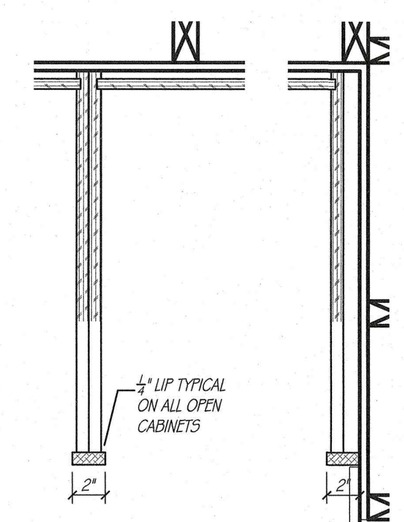
CABINET DETAIL SCALE: 1 1/2" = 1'-0"
