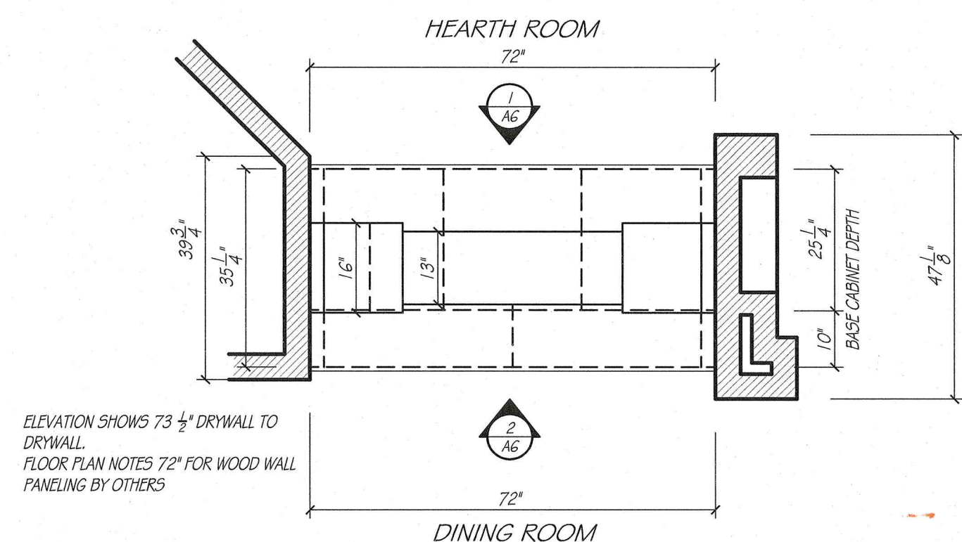
HEARTH ROOM / DINING SCALE: 1/2" = 1'-0"
