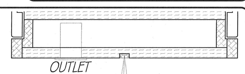
CROWN DETAIL ✓ SCALE: 3" = 1'-0"
