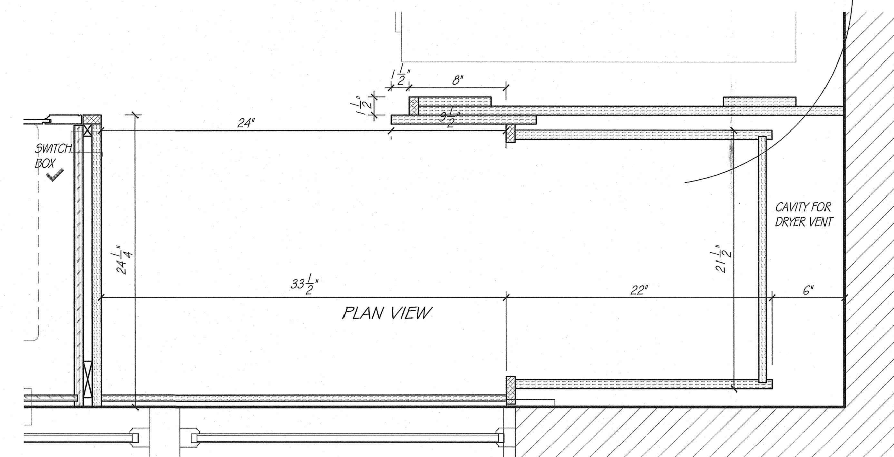
6 CABINET DETAIL SCALE: 1 1/2" = 1'-0"
