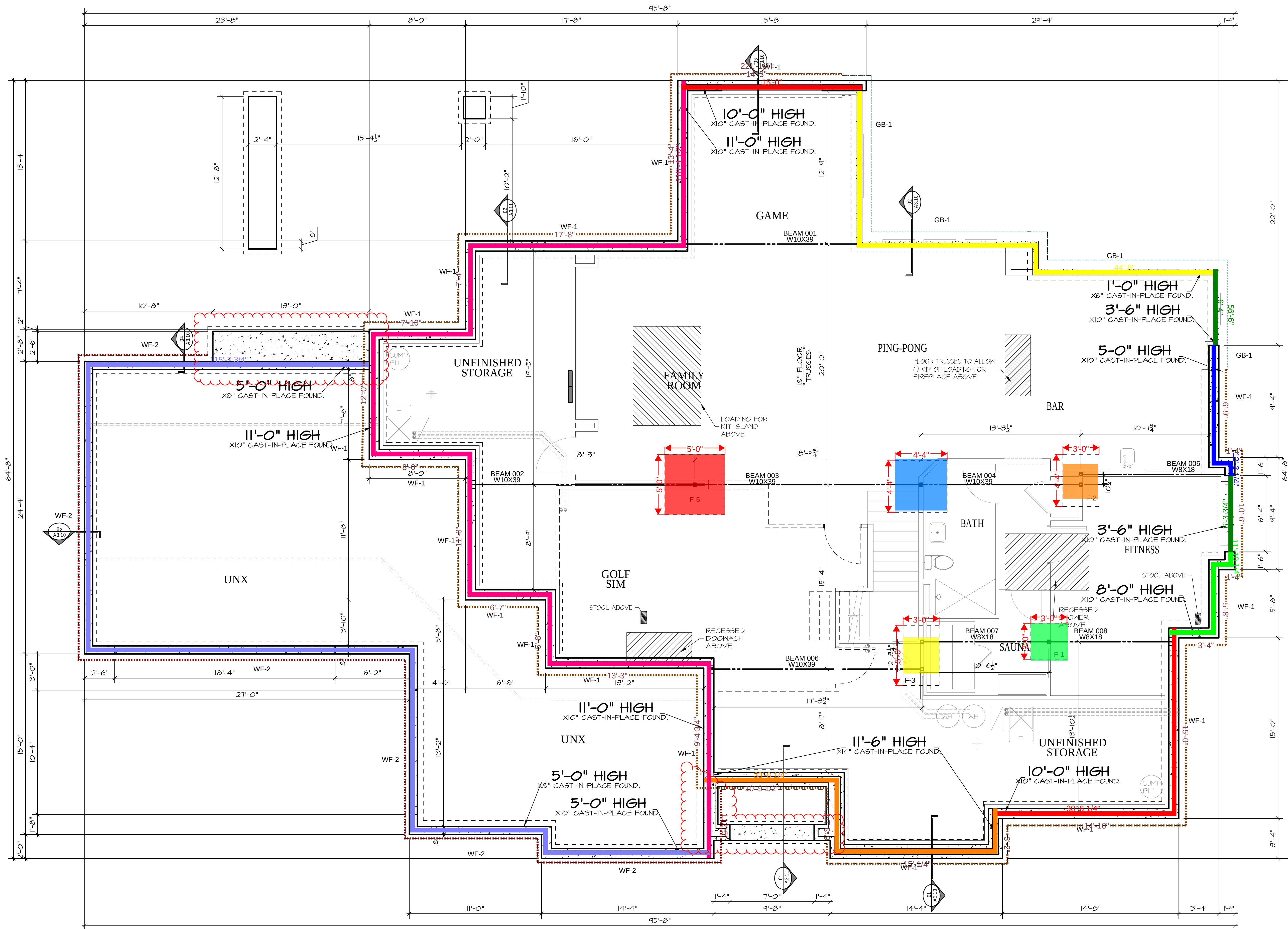
FOUNDATION PLAN
