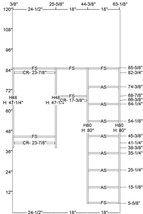
Wall Elevation A
