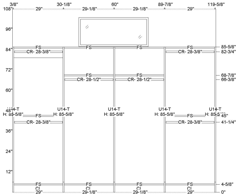
Wall Elevation C
