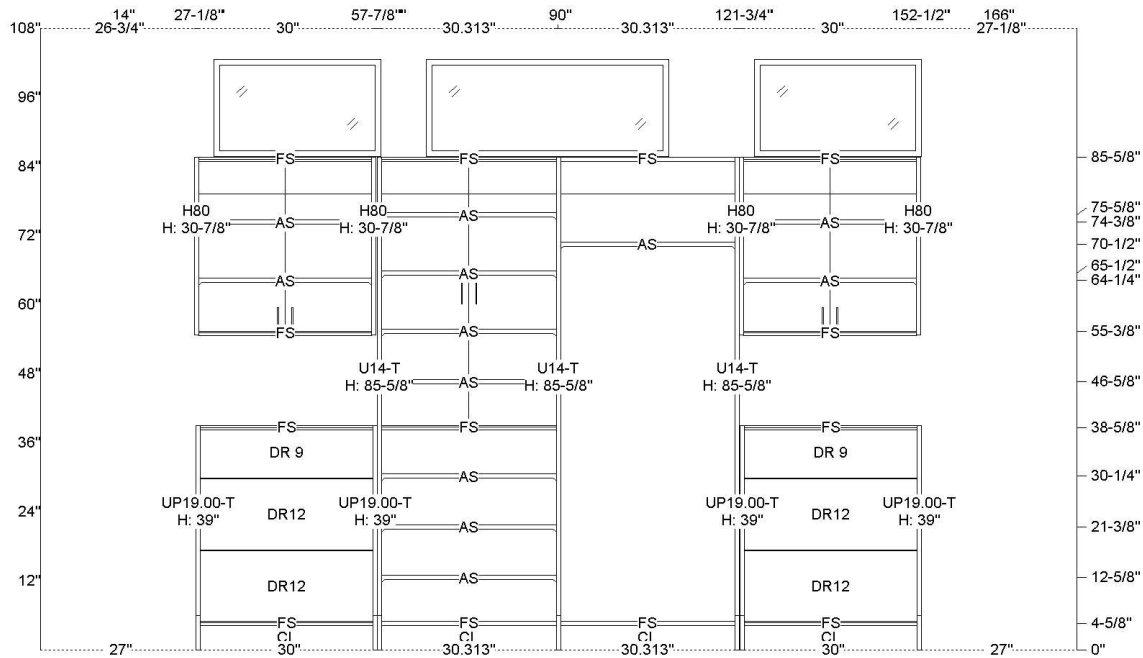
Wall Elevation B
