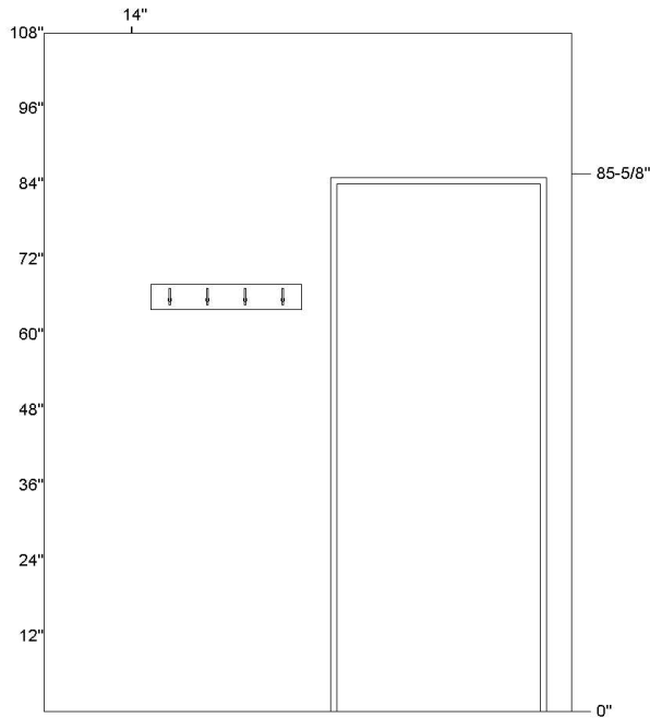
Wall Elevation D
