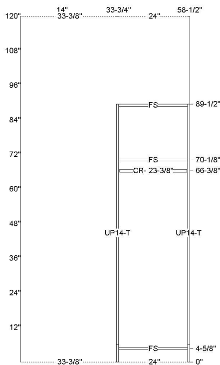
Wall Elevation B
