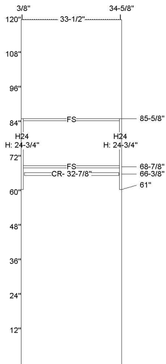
Wall Elevation A
