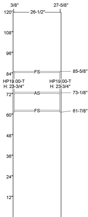
Wall Elevation A
