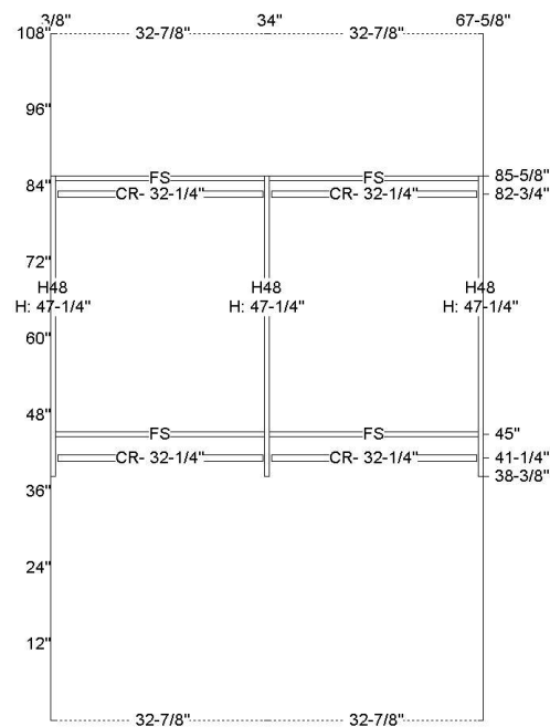
Wall Elevation B
