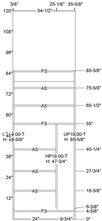
Wall Elevation A
