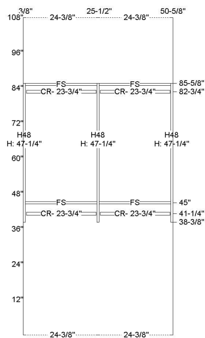
Wall Elevation B
