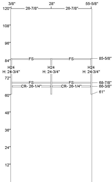
Wall Elevation A
