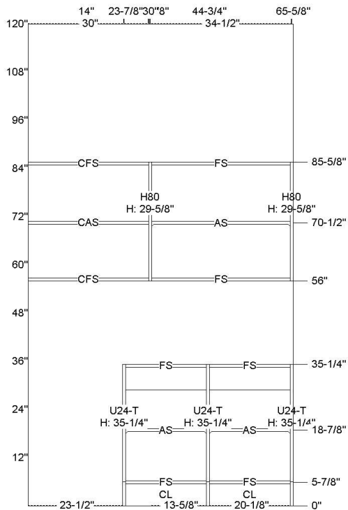
Wall Elevation C
