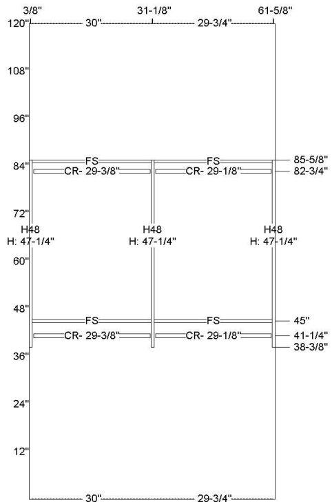
Wall Elevation C
