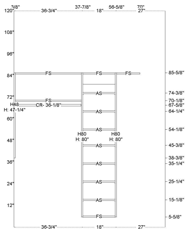
Wall Elevation B
