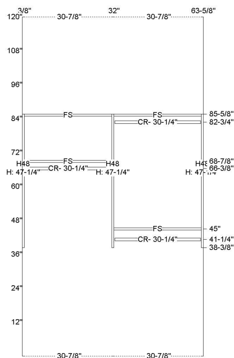
Wall Elevation B
