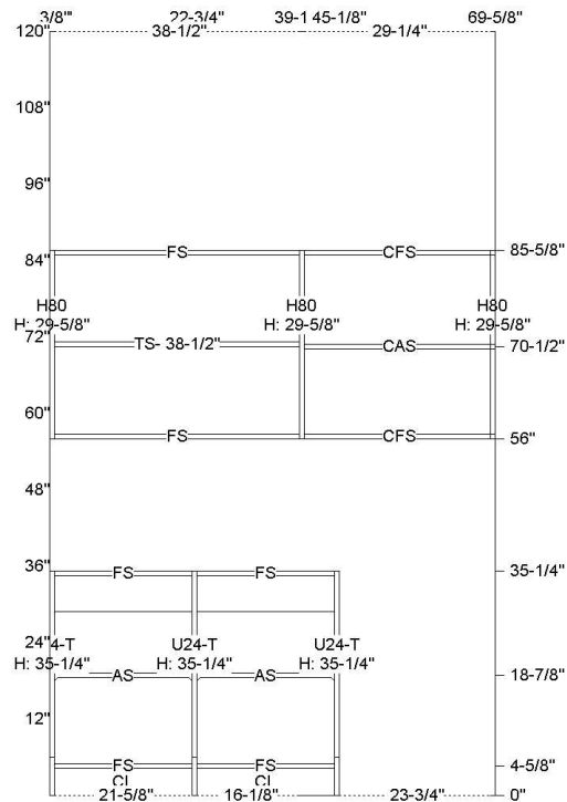
Wall Elevation B
