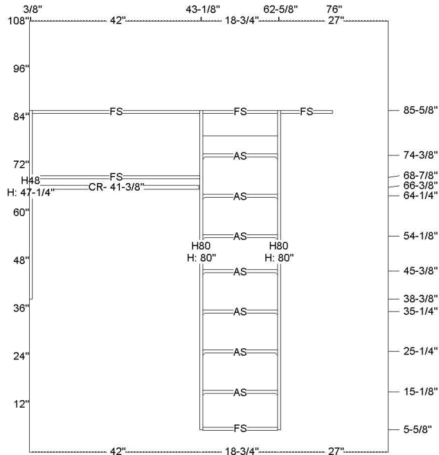
Wall Elevation A
