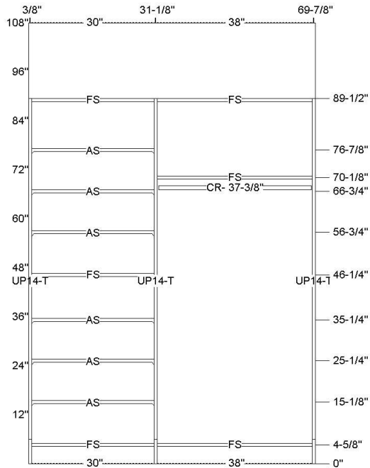
Wall Elevation A
