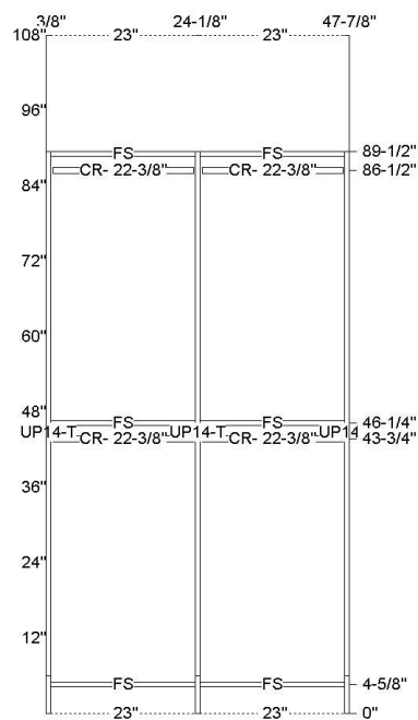
Wall Elevation B
