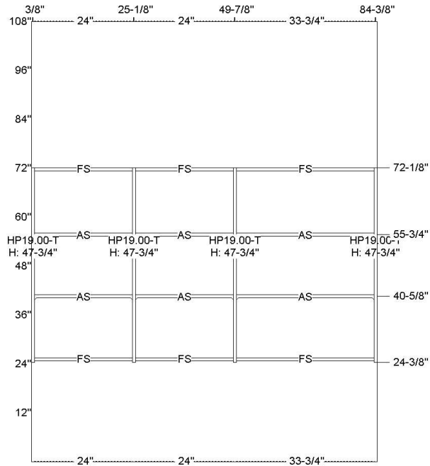
Wall Elevation A
