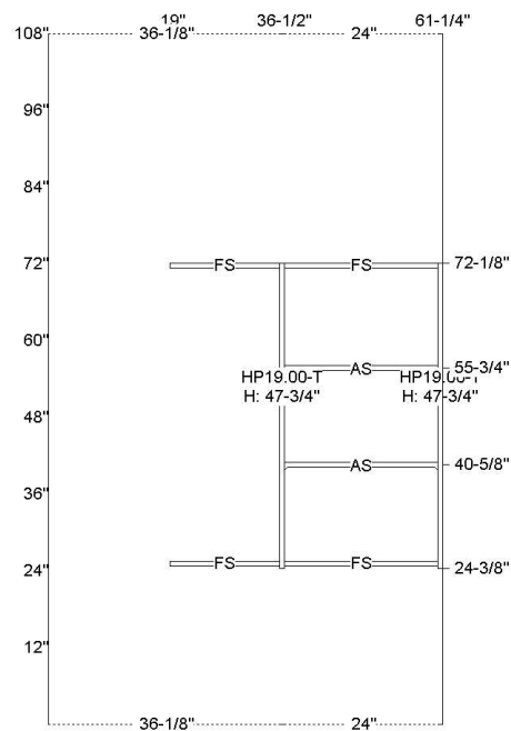
Wall Elevation B
