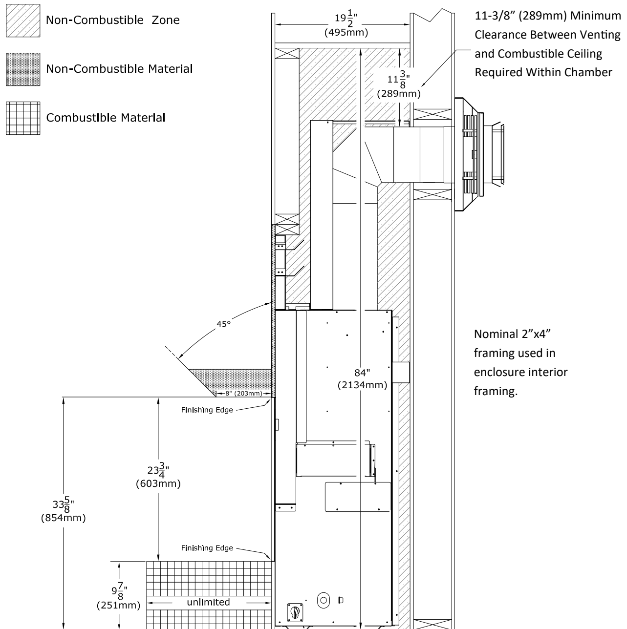
Figure 5.3 - Non-Combustible Mantel Projections - Standard Installation Design
