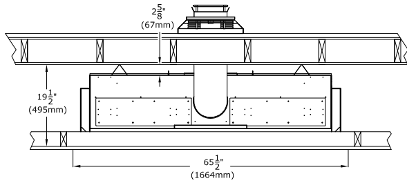
TYPICAL HORIZONTAL INSTALLATION
