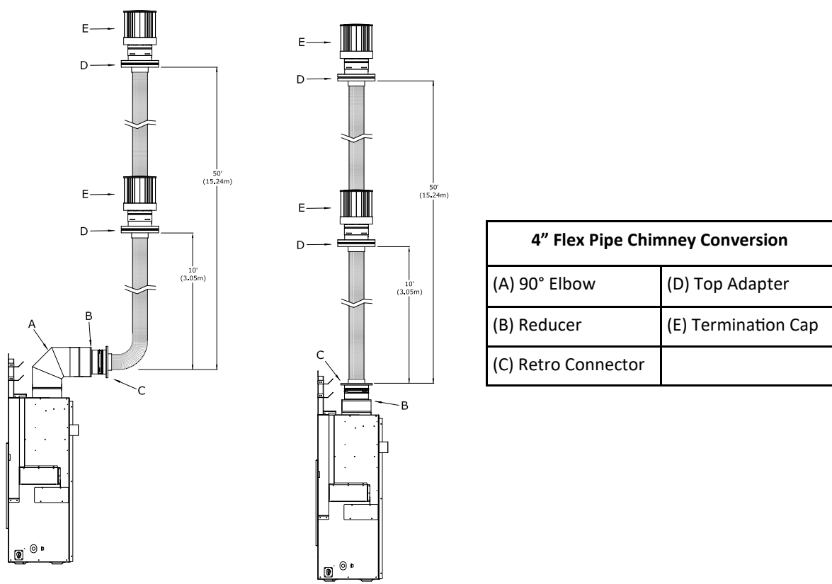
Figure 8.8 - Class A Chimney / Masonry Chimney
