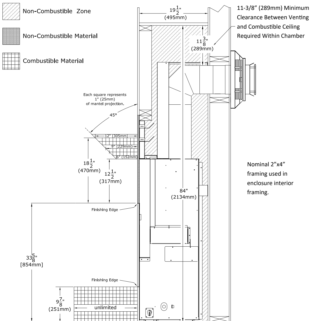
Figure 5.2 - Combustible Mantel Projections - Standard Installation Design
