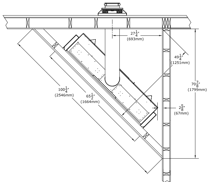
TYPICAL CORNER INSTALLATION
