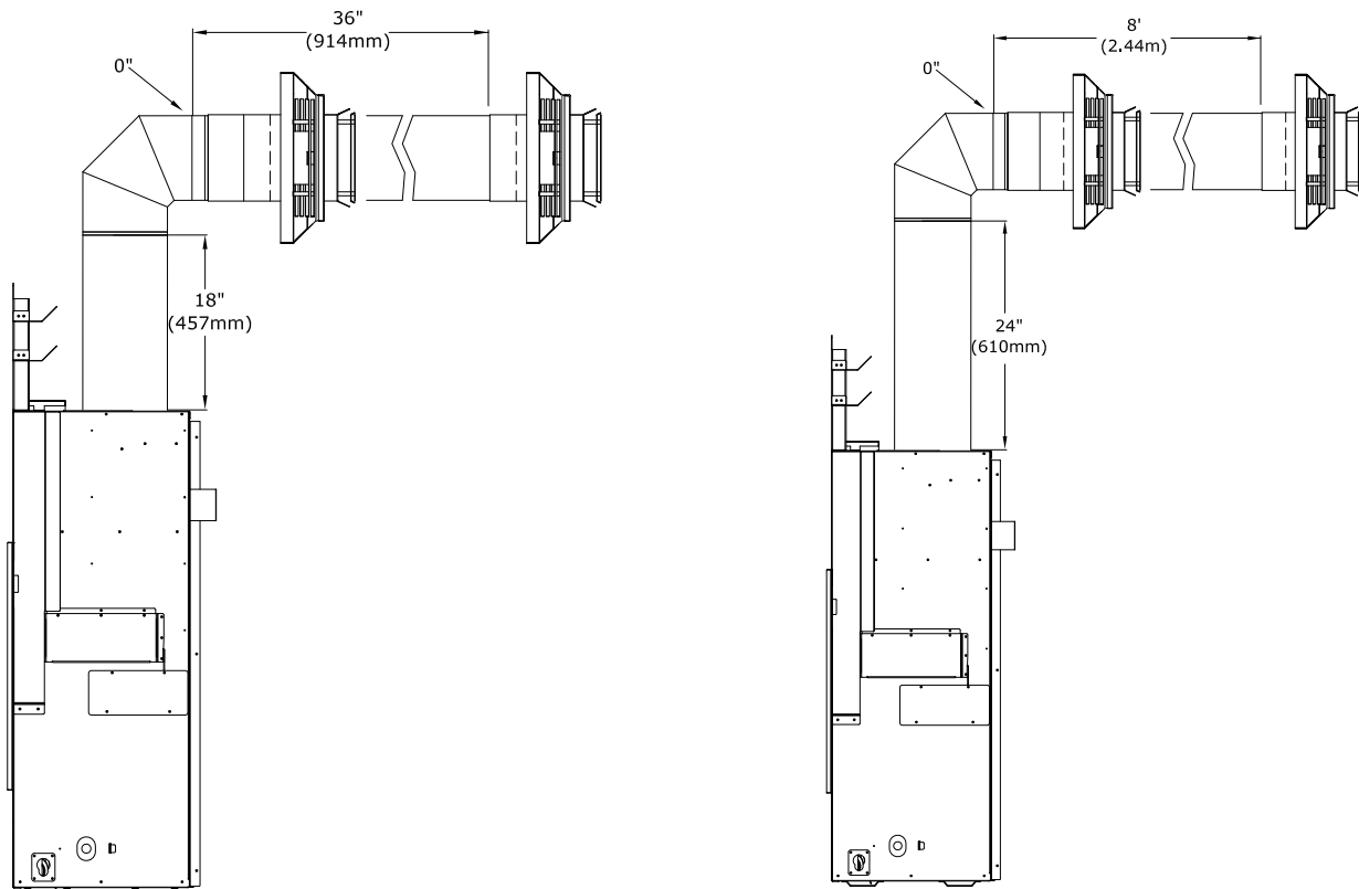
Figure 8.4 - Horizontal 5" x 8" Vent Pipe
