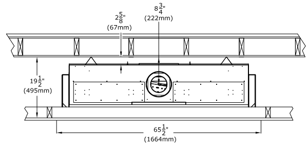
TYPICAL VERTICAL INSTALLATION
