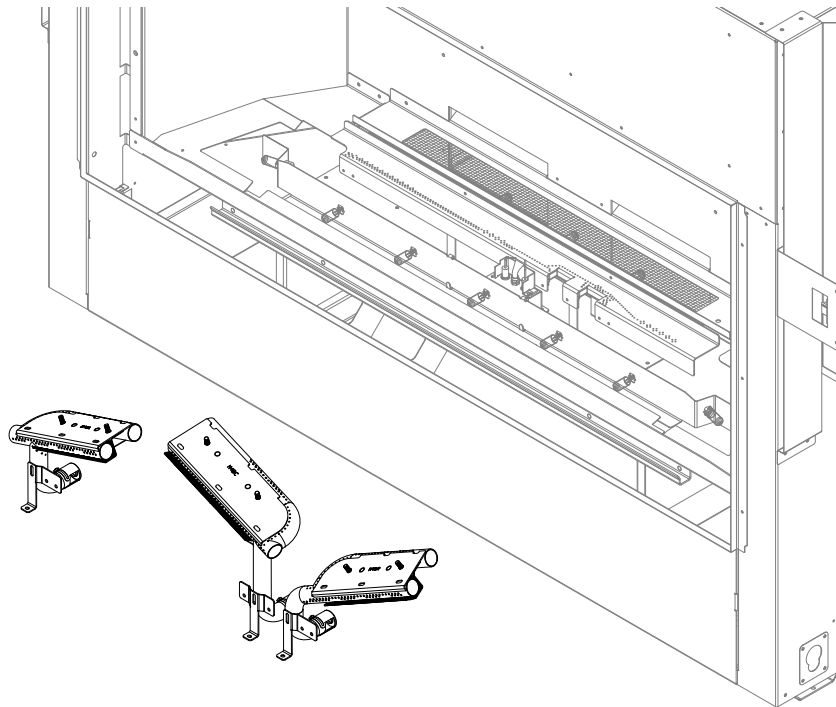
Figure 9.4 - Left, Center, and Right Burner Removal
