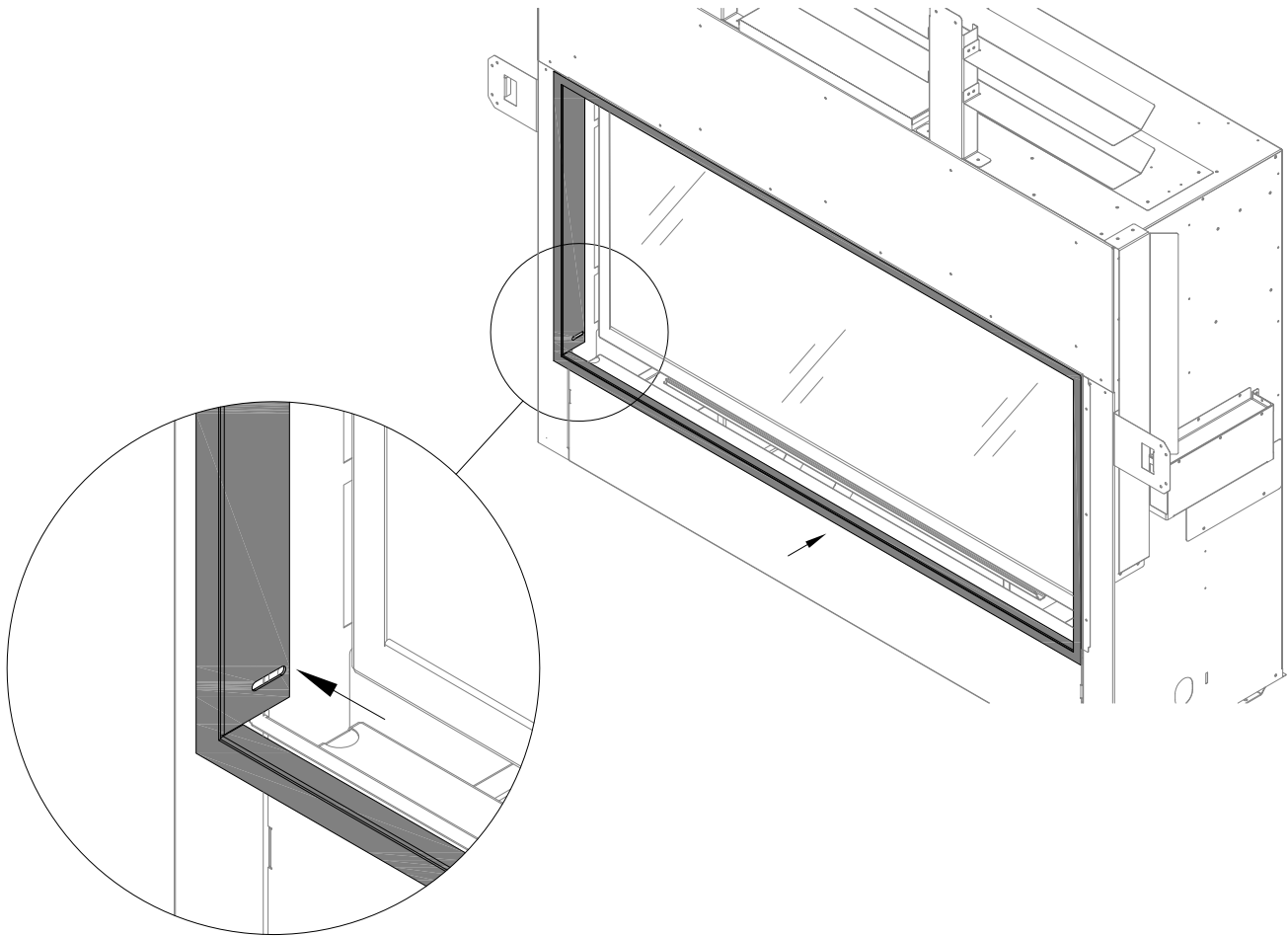
Figure 5.7 - Rectangle Surround Installation
