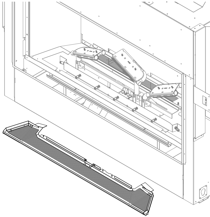
Figure 9.3 - Ember Media Tray Removal
