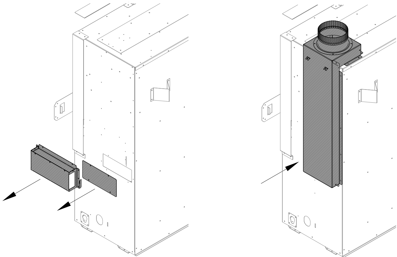
Figure 4.4 - HTK Air Chute Installation
