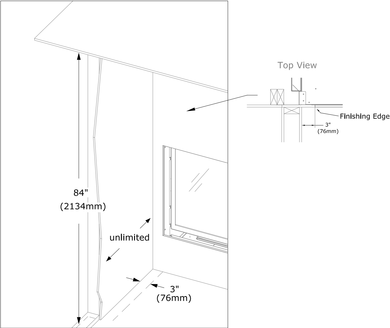
Figure 5.5 - Combustible Sidewall Projection
