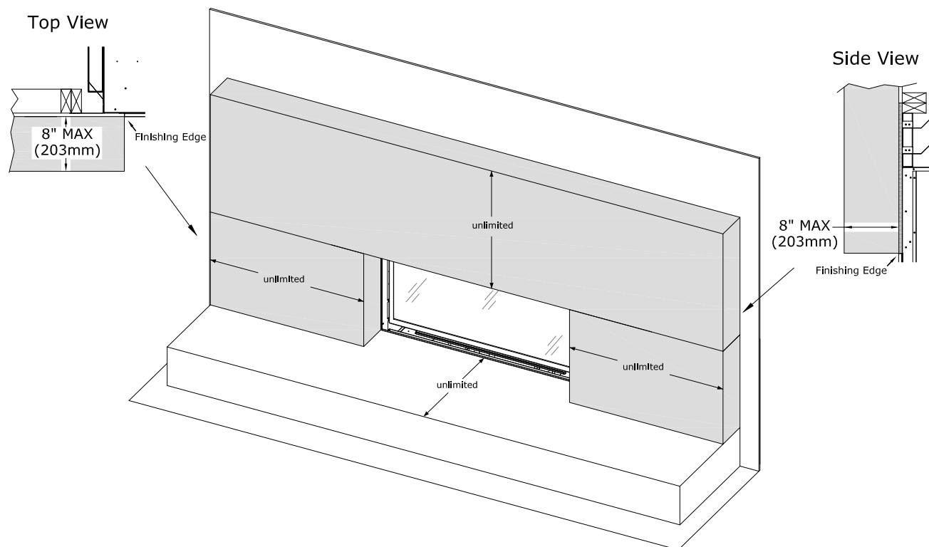
Figure 5.4 - Non-Combustible Surround Projection
