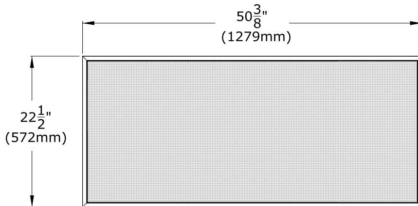
Safety Barrier Screen NK48TL-ES
