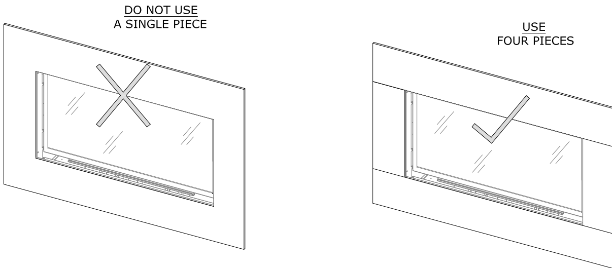
Figure 5.1 - Marble Installation Example
