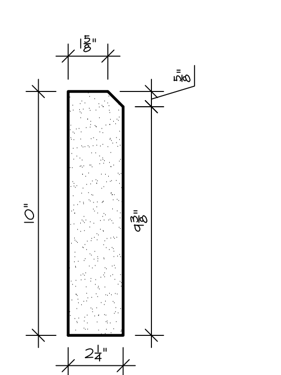
SECTION 3" SCALE
