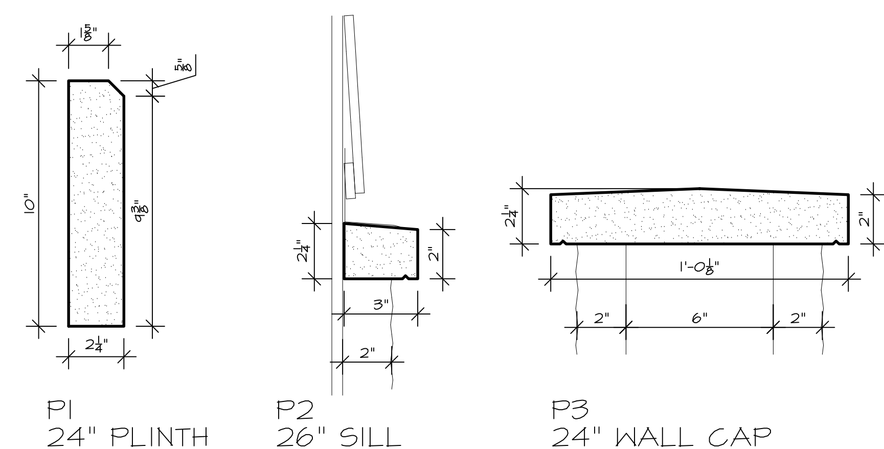
SECTION PRECAST PROFILES 3" SCALE
