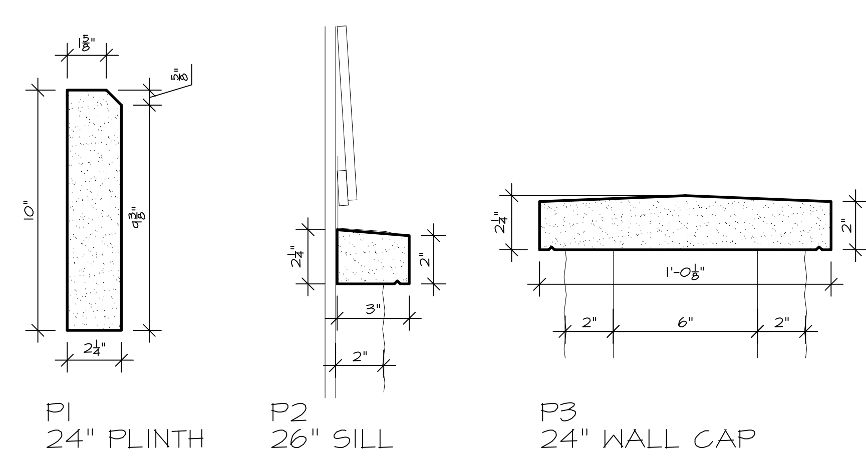
SECTION PRECAST PROFILES 3" SCALE
