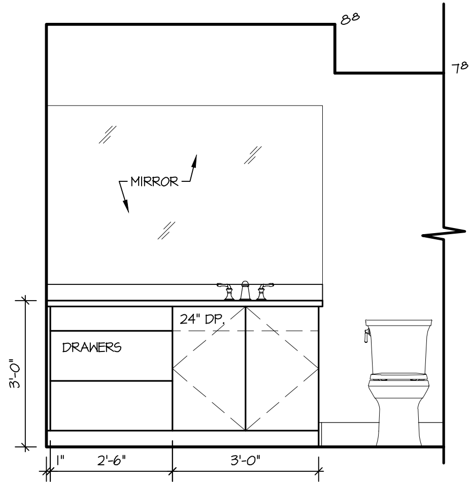
03 BATH #3 1/2" SCALE
