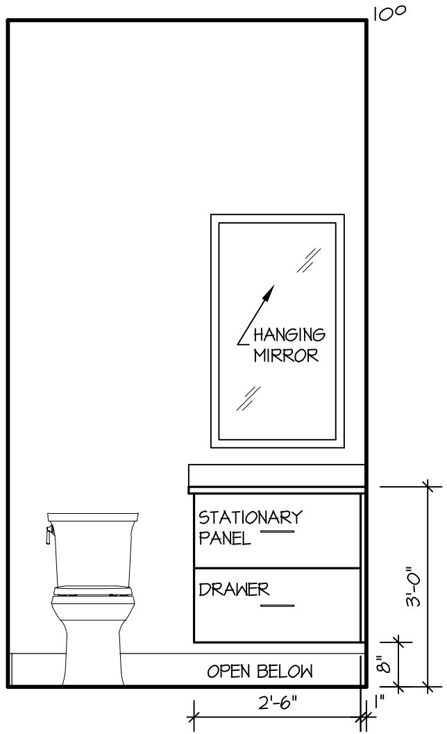
02 POWDER 1/2" SCALE
