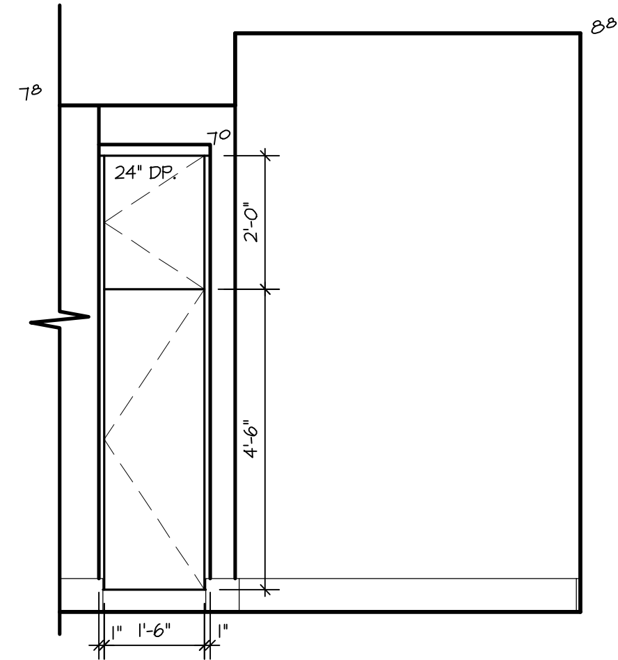
04 BATH #3 1/2" SCALE
