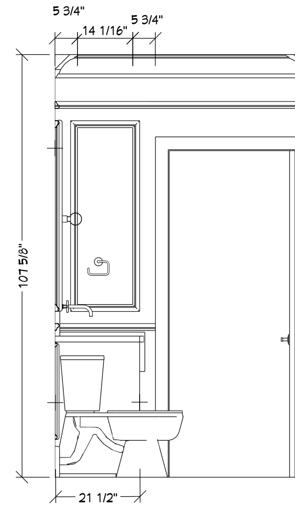
Elevation 24 POWDER
