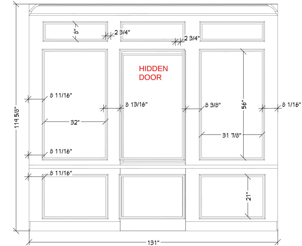
ENTRY Elevation 2
