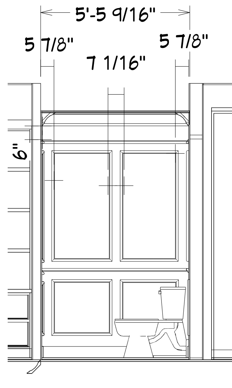
Elevation 5 POWDER
