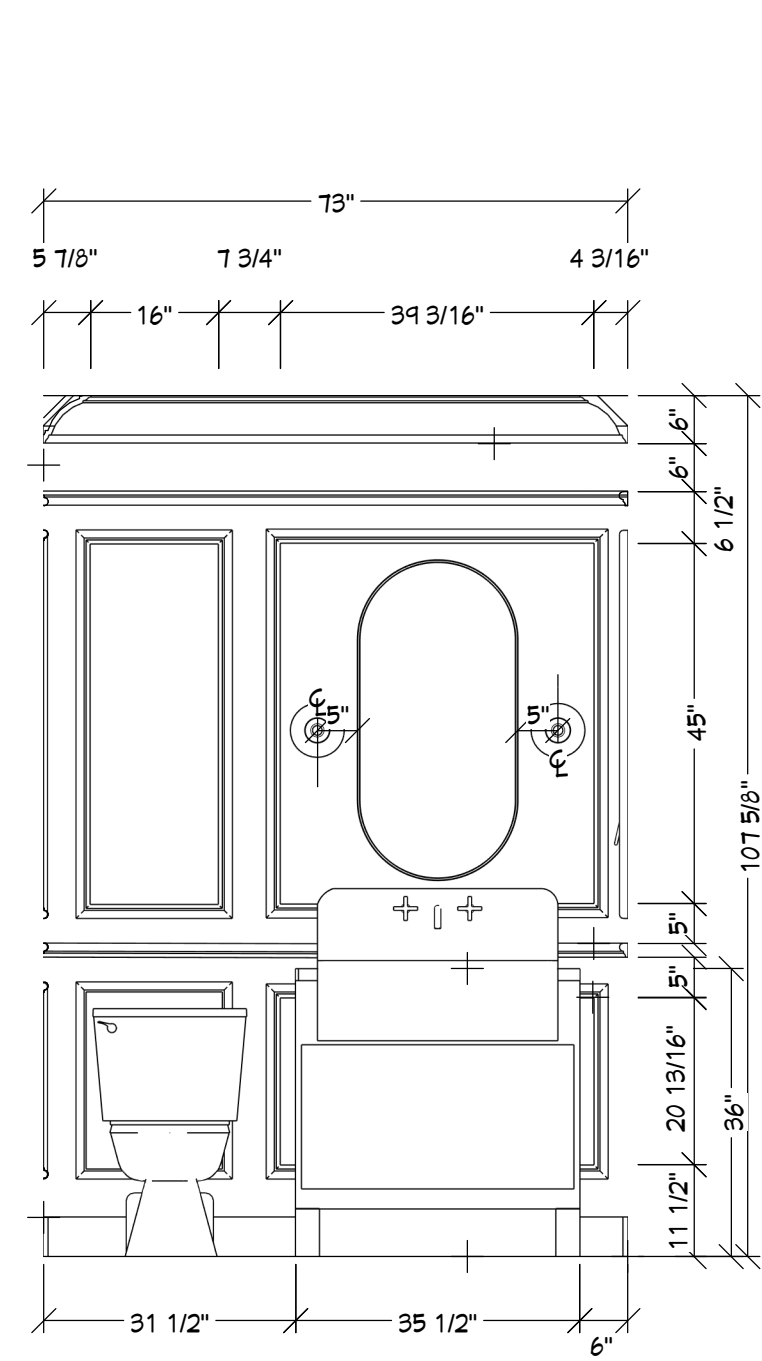
Elevation 22 POWDER
