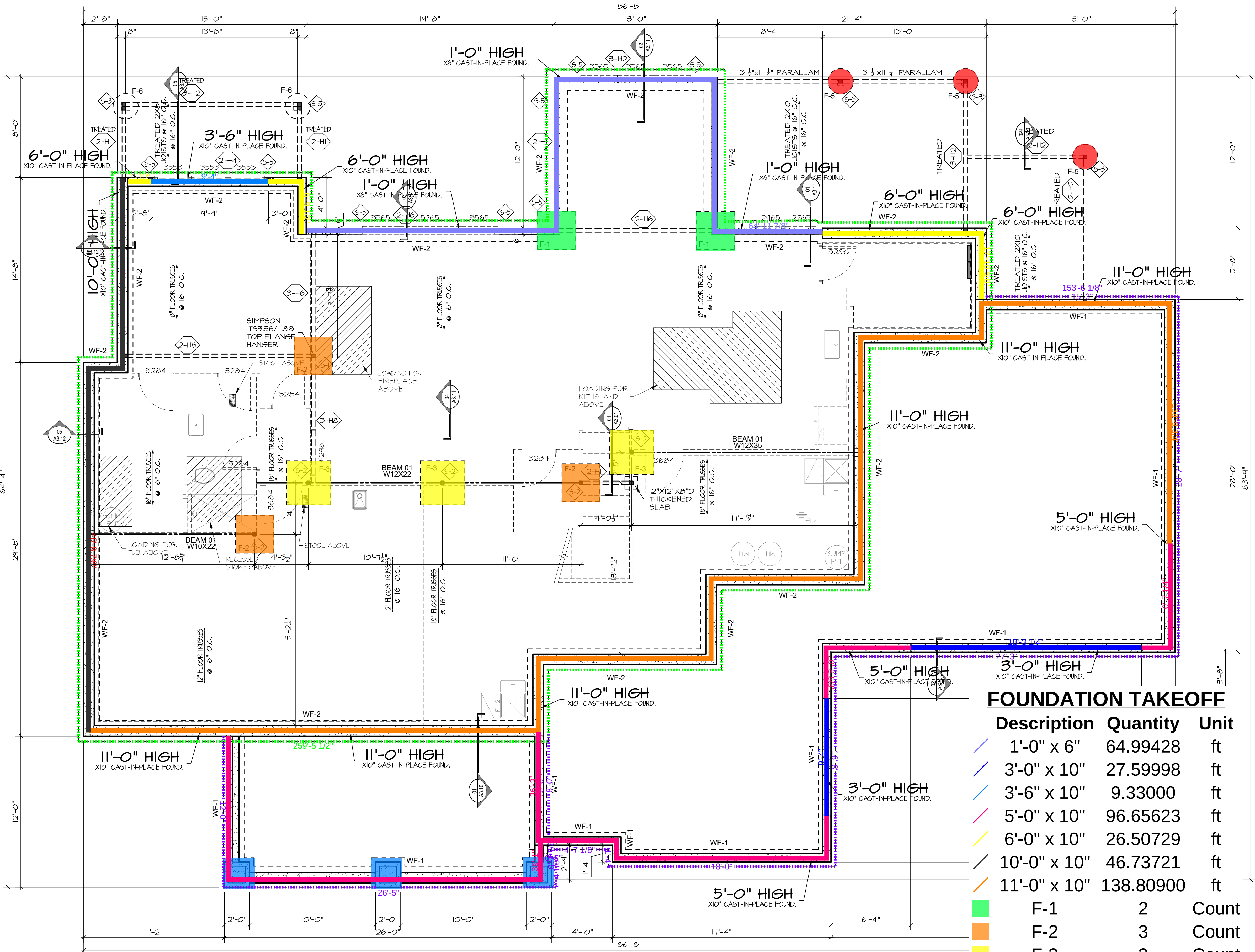
FOUNDATION PLAN
