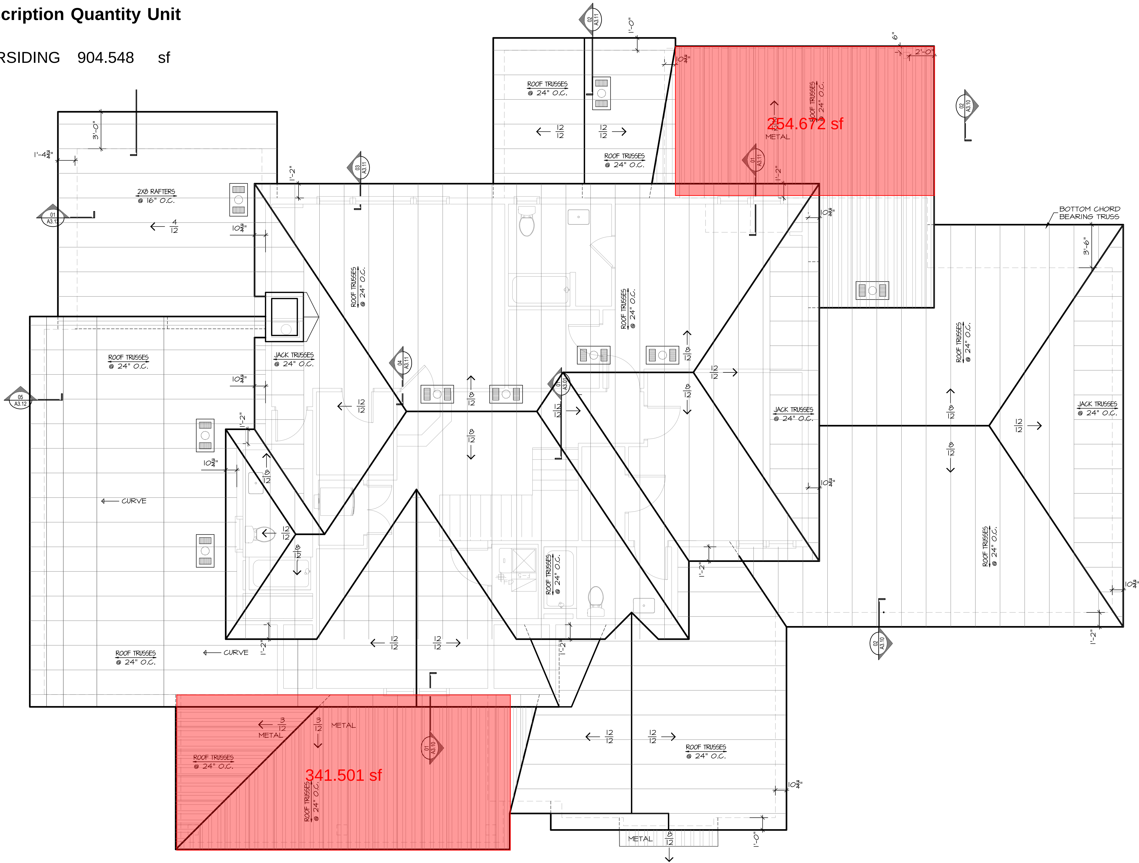
ROOF PLAN
