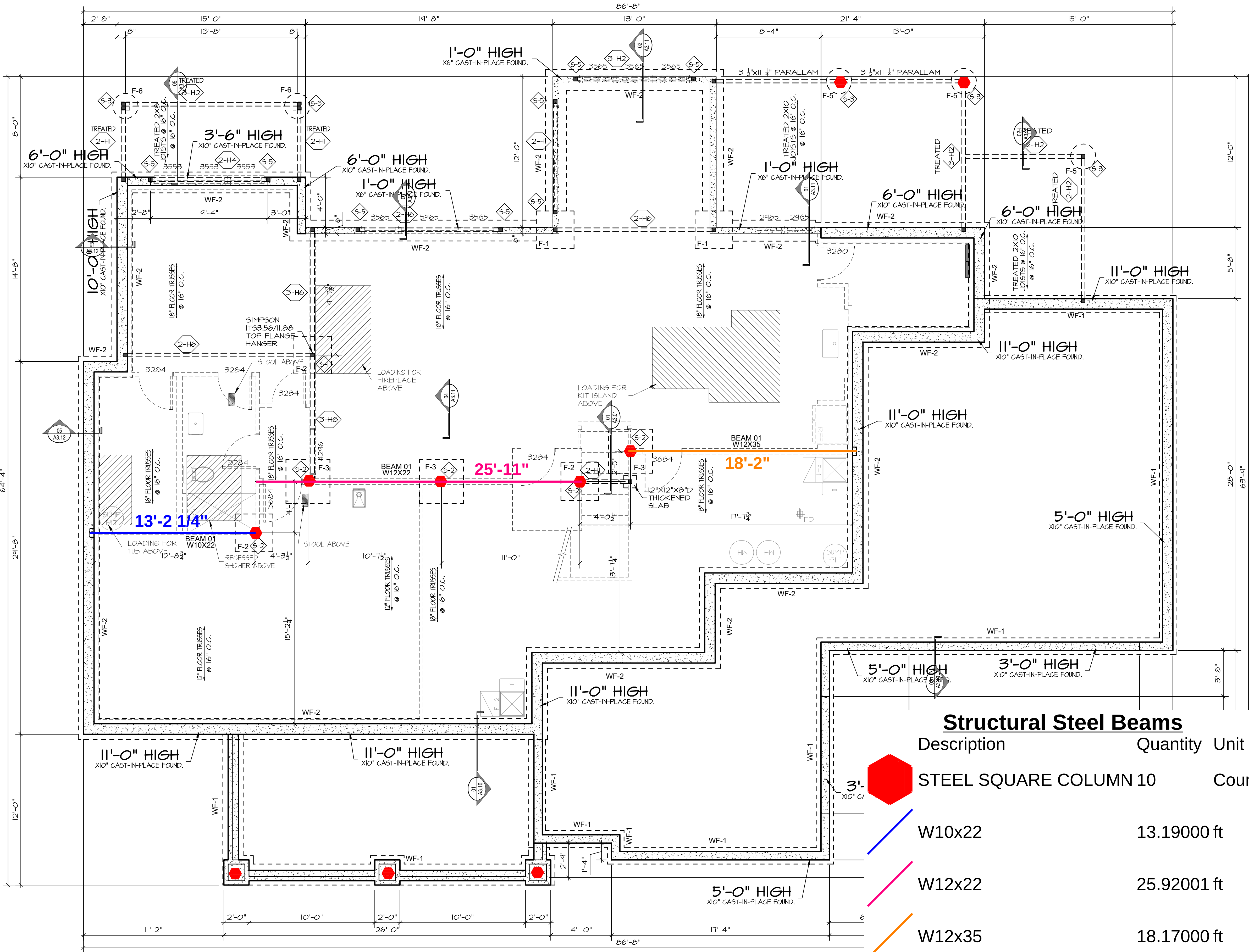
FOUNDATION PLAN
